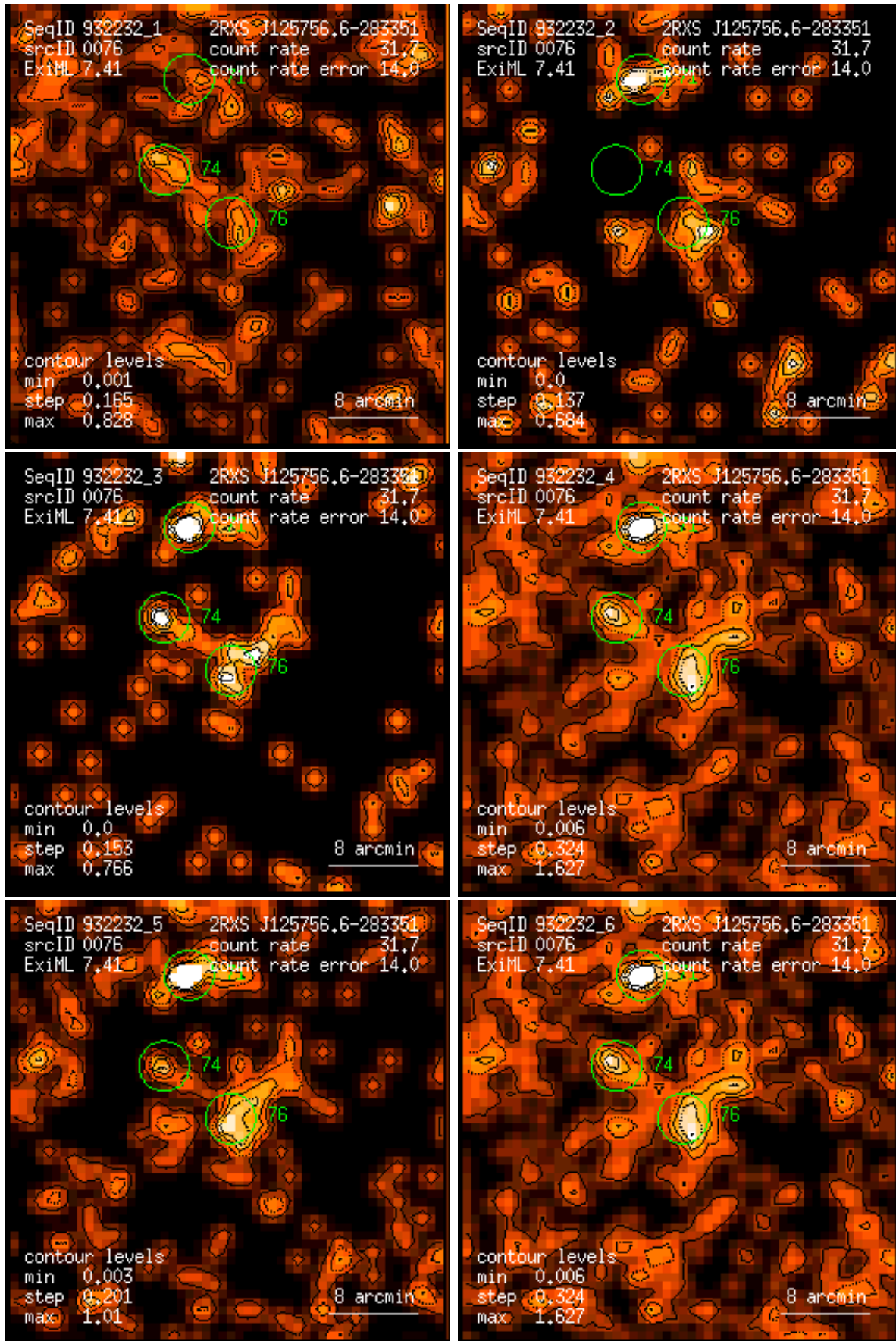
Figure 76: RASS 932232: detection 0076: band rate images, Gaussian filter: (1) PSPC channels 11 – 41, (2) 52 – 90, (3) 91 – 201, (4) 11 – 235, (5) 52 – 201, (6) 11 – 201. Broad band rates in counts/ks. Band rate contour levels in counts/ks/arcmin 2 .
