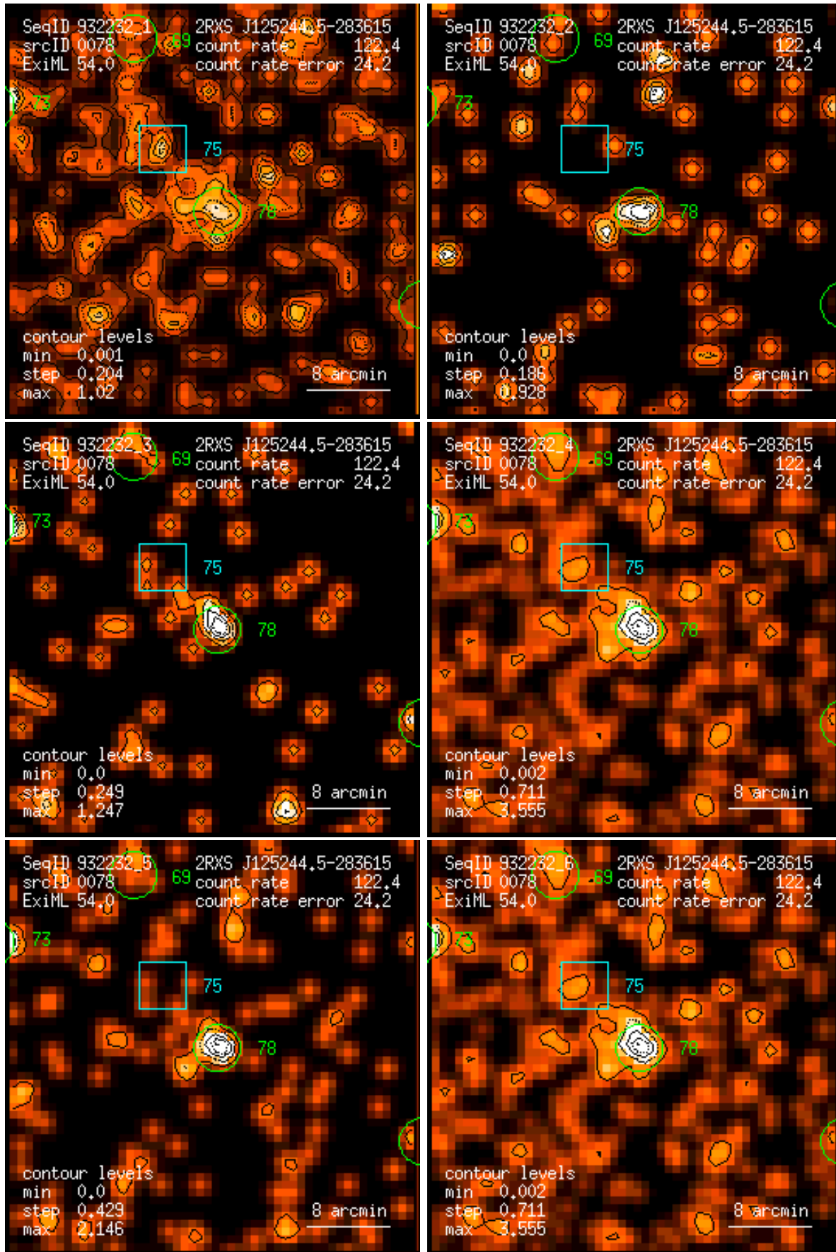
Figure 78: RASS 932232: detection 0078: band rate images, Gaussian filter: (1) PSPC channels 11 – 41, (2) 52 – 90, (3) 91 – 201, (4) 11 – 235, (5) 52 – 201, (6) 11 – 201. Broad band rates in counts/ks. Band rate contour levels in counts/ks/arcmin 2 .
