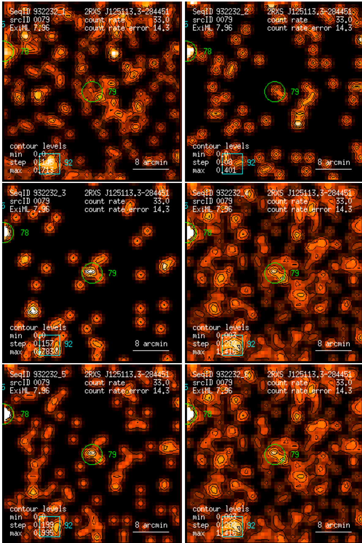
Figure 79: RASS 932232: detection 0079: band rate images, Gaussian filter: (1) PSPC channels 11 – 41, (2) 52 – 90, (3) 91 – 201, (4) 11 – 235, (5) 52 – 201, (6) 11 – 201. Broad band rates in counts/ks. Band rate contour levels in counts/ks/arcmin 2 .
