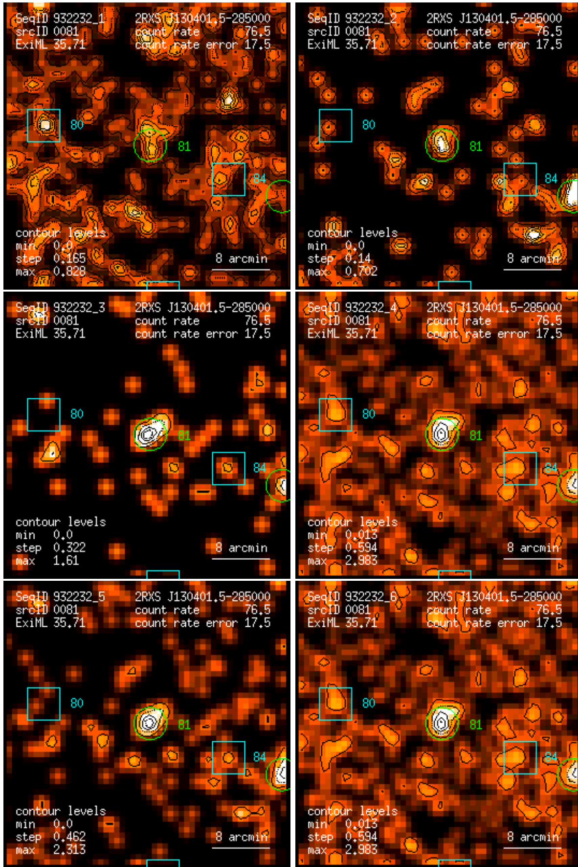
Figure 81: RASS 932232: detection 0081: band rate images, Gaussian filter: (1) PSPC channels 11 – 41, (2) 52 – 90, (3) 91 – 201, (4) 11 – 235, (5) 52 – 201, (6) 11 – 201. Broad band rates in counts/ks. Band rate contour levels in counts/ks/arcmin 2 .
