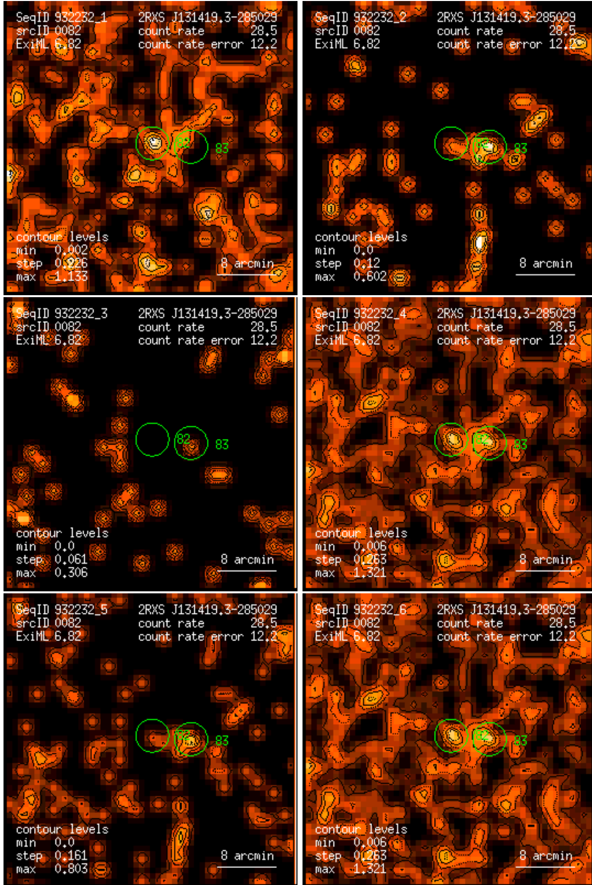
Figure 82: RASS 932232: detection 0082: band rate images, Gaussian filter: (1) PSPC channels 11 – 41, (2) 52 – 90, (3) 91 – 201, (4) 11 – 235, (5) 52 – 201, (6) 11 – 201. Broad band rates in counts/ks. Band rate contour levels in counts/ks/arcmin 2 .
