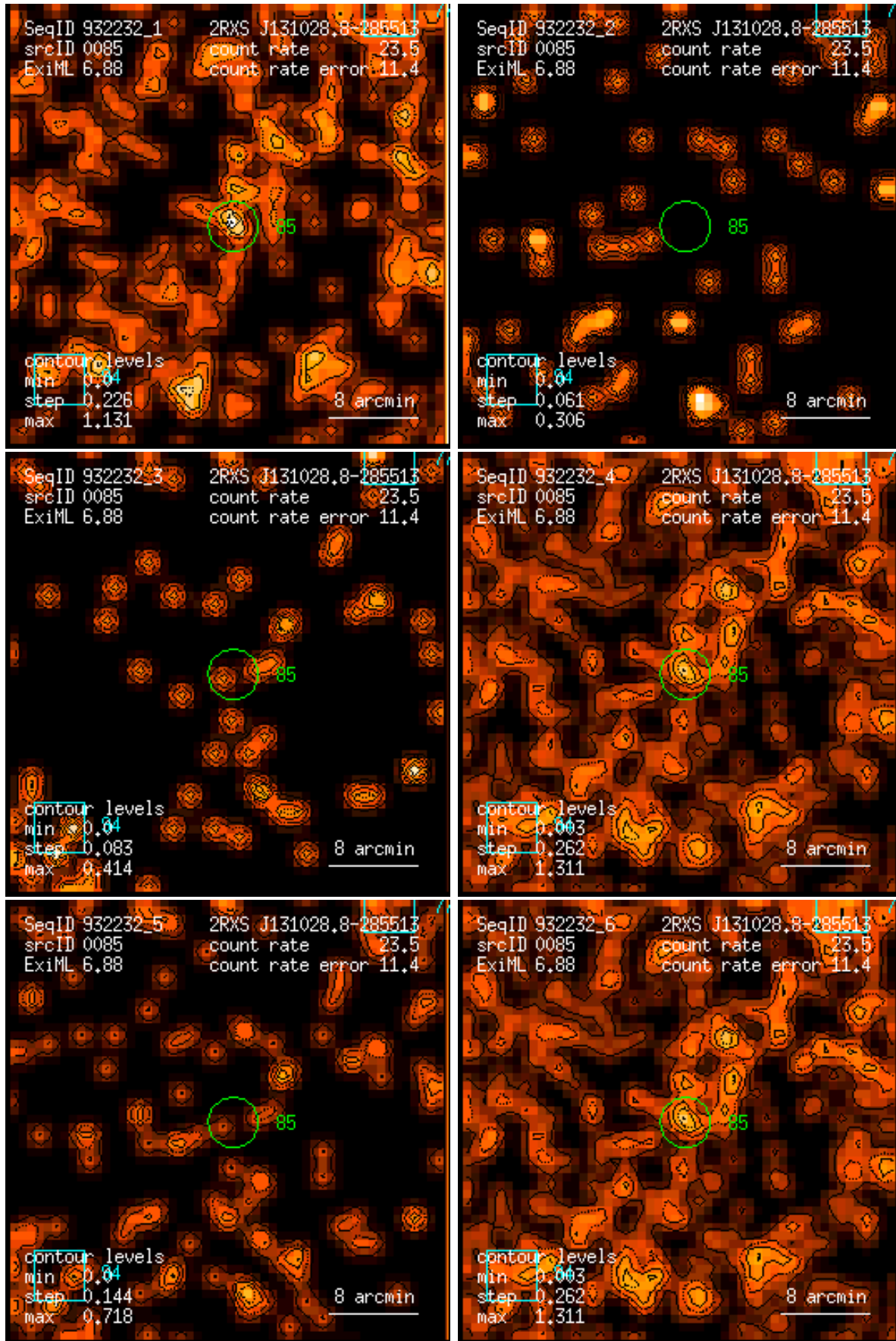
Figure 85: RASS 932232: detection 0085: band rate images, Gaussian filter: (1) PSPC channels 11 – 41, (2) 52 – 90, (3) 91 – 201, (4) 11 – 235, (5) 52 – 201, (6) 11 – 201. Broad band rates in counts/ks. Band rate contour levels in counts/ks/arcmin 2 .
