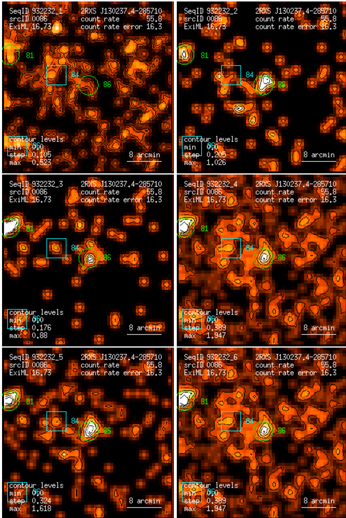
Figure 86: RASS 932232: detection 0086: band rate images, Gaussian filter: (1) PSPC channels 11 – 41, (2) 52 – 90, (3) 91 – 201, (4) 11 – 235, (5) 52 – 201, (6) 11 – 201. Broad band rates in counts/ks. Band rate contour levels in counts/ks/arcmin 2 .
