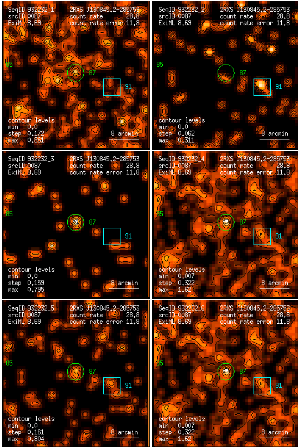
Figure 87: RASS 932232: detection 0087: band rate images, Gaussian filter: (1) PSPC channels 11 – 41, (2) 52 – 90, (3) 91 – 201, (4) 11 – 235, (5) 52 – 201, (6) 11 – 201. Broad band rates in counts/ks. Band rate contour levels in counts/ks/arcmin 2 .
