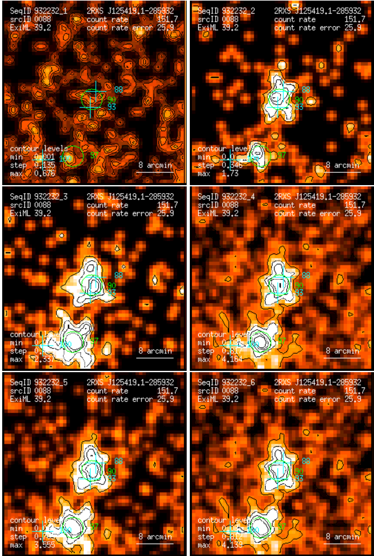
Figure 88: RASS 932232: detection 0088: band rate images, Gaussian filter: (1) PSPC channels 11 – 41, (2) 52 – 90, (3) 91 – 201, (4) 11 – 235, (5) 52 – 201, (6) 11 – 201. Broad band rates in counts/ks. Band rate contour levels in counts/ks/arcmin 2 .
