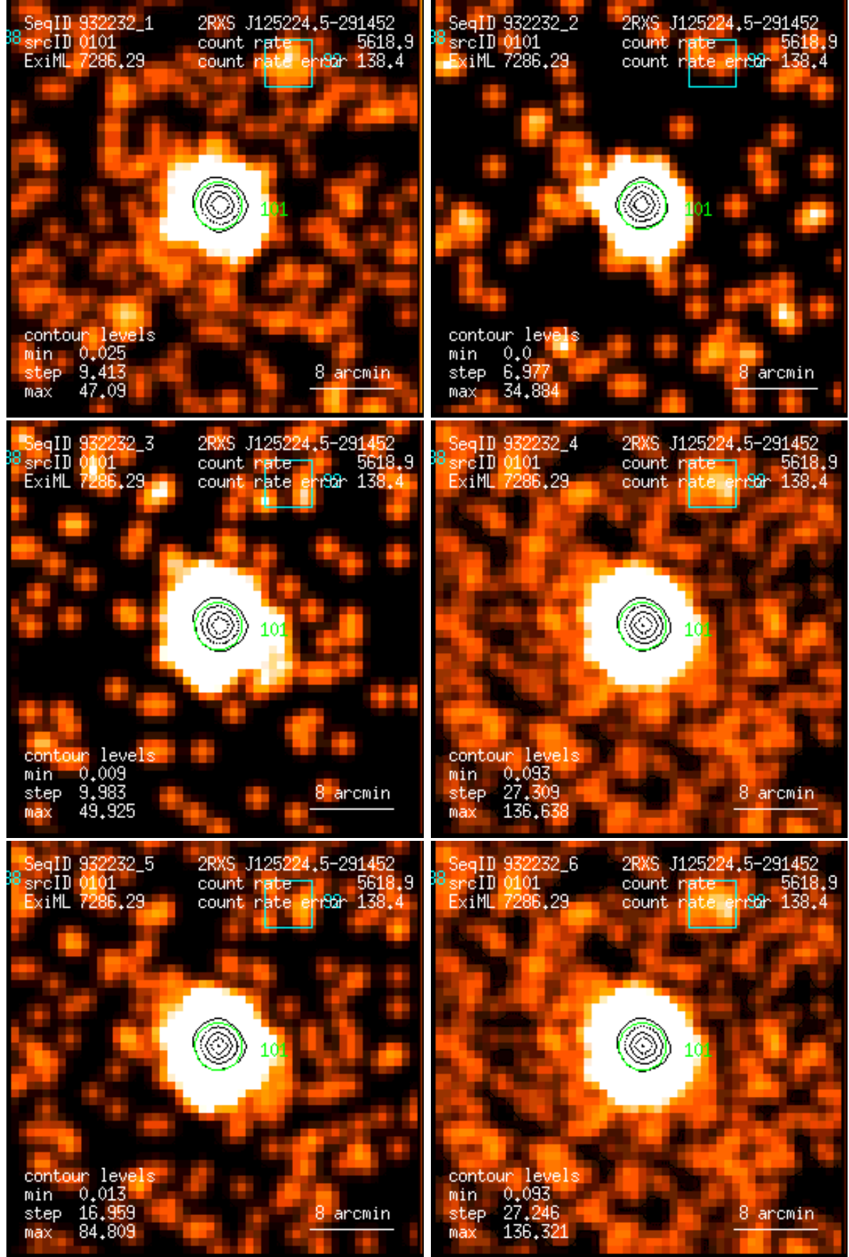
Figure 101: RASS 932232: detection 0101: band rate images, Gaussian filter: (1) PSPC channels 11 – 41, (2) 52 – 90, (3) 91 – 201, (4) 11 – 235, (5) 52 – 201, (6) 11 – 201. Broad band rates in counts/ks. Band rate contour levels in counts/ks/arcmin 2 .
