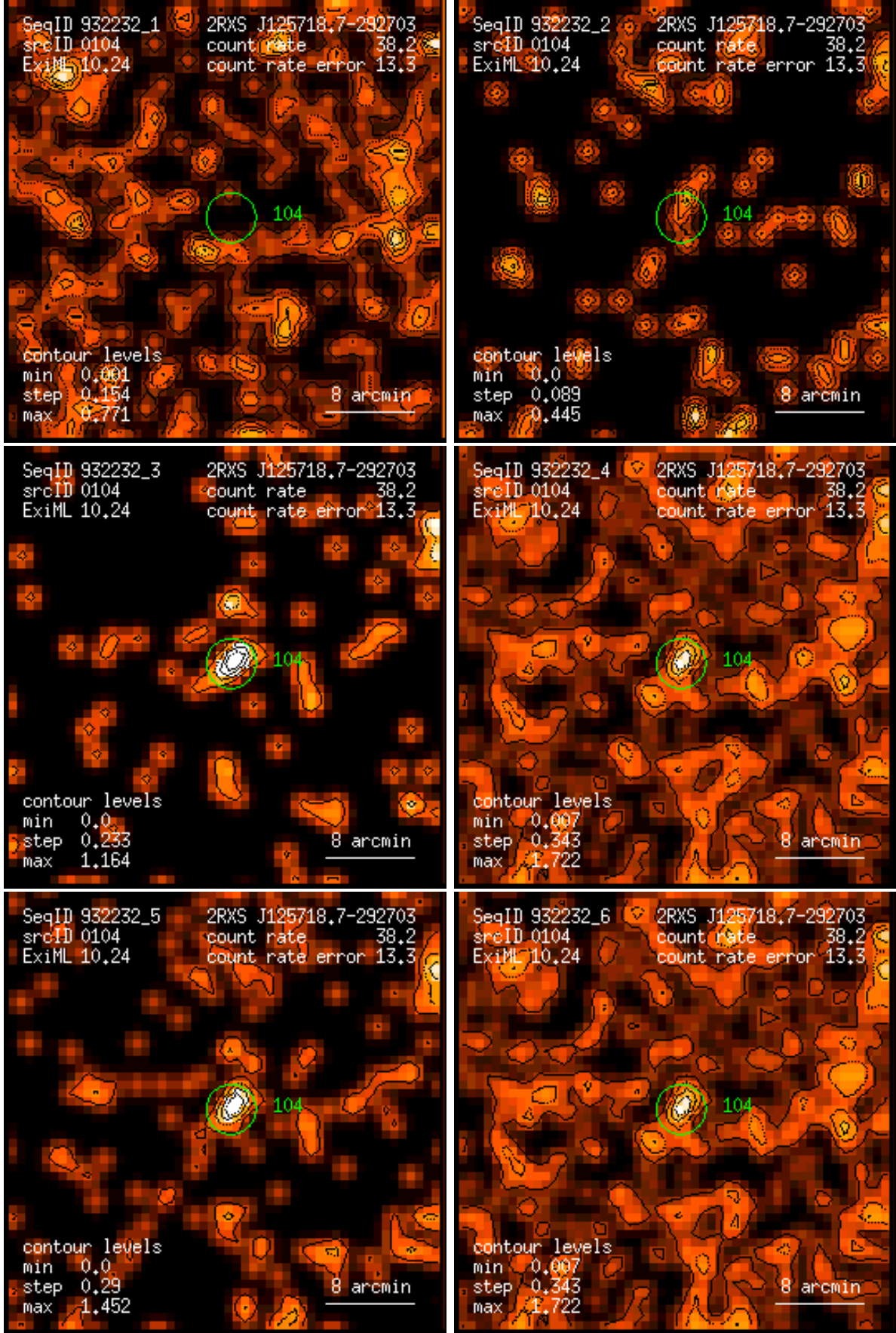
Figure 104: RASS 932232: detection 0104: band rate images, Gaussian filter: (1) PSPC channels 11 – 41, (2) 52 – 90, (3) 91 – 201, (4) 11 – 235, (5) 52 – 201, (6) 11 – 201. Broad band rates in counts/ks. Band rate contour levels in counts/ks/arcmin 2 .
