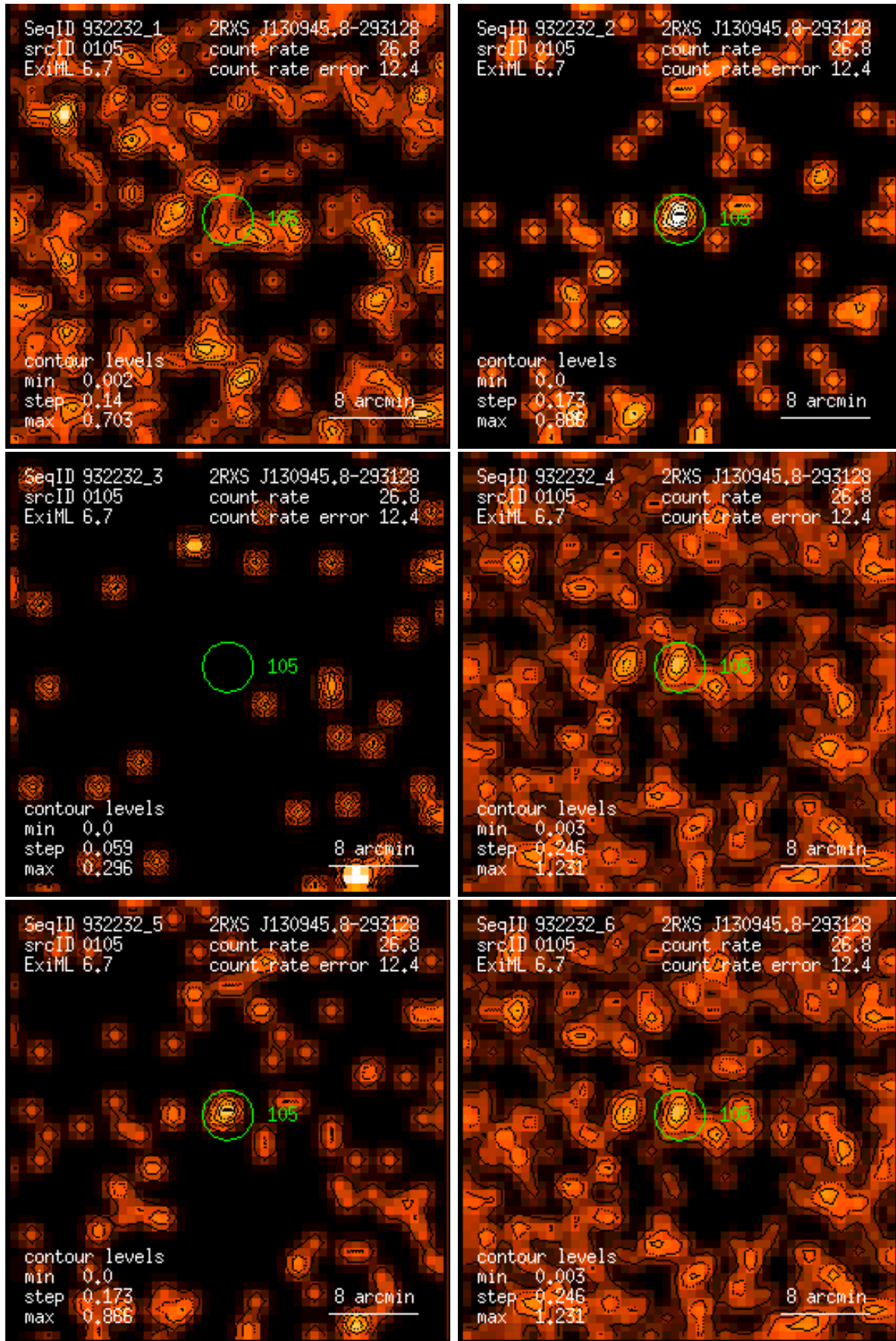
Figure 105: RASS 932232: detection 0105: band rate images, Gaussian filter: (1) PSPC channels 11 – 41, (2) 52 – 90, (3) 91 – 201, (4) 11 – 235, (5) 52 – 201, (6) 11 – 201. Broad band rates in counts/ks. Band rate contour levels in counts/ks/arcmin 2 .
