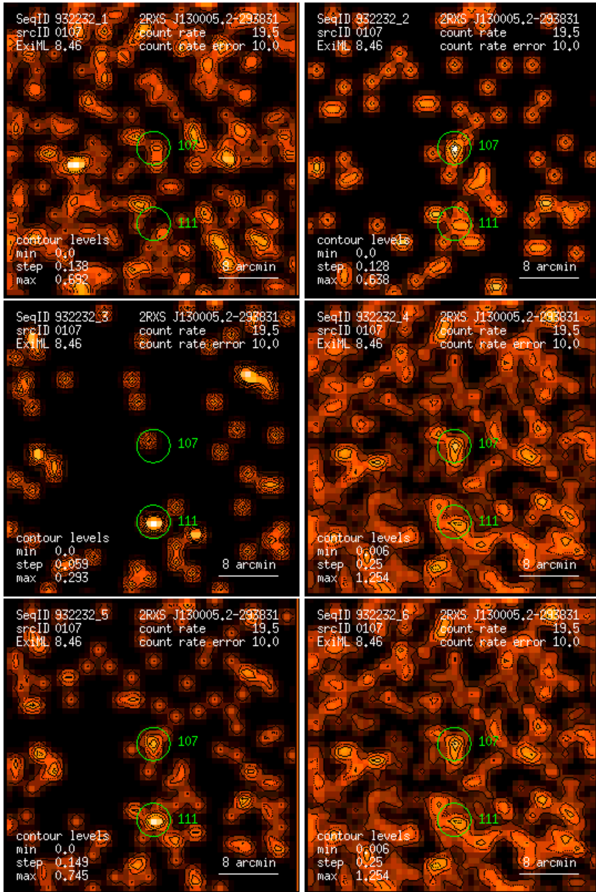
Figure 107: RASS 932232: detection 0107: band rate images, Gaussian filter: (1) PSPC channels 11 – 41, (2) 52 – 90, (3) 91 – 201, (4) 11 – 235, (5) 52 – 201, (6) 11 – 201. Broad band rates in counts/ks. Band rate contour levels in counts/ks/arcmin 2 .
