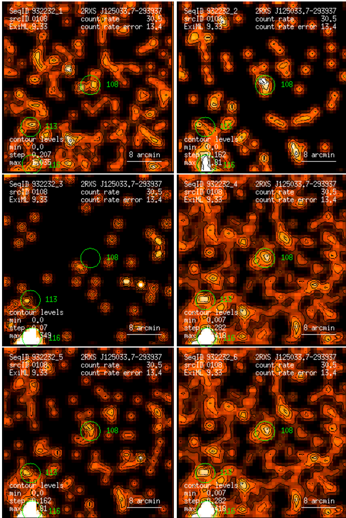
Figure 108: RASS 932232: detection 0108: band rate images, Gaussian filter: (1) PSPC channels 11 – 41, (2) 52 – 90, (3) 91 – 201, (4) 11 – 235, (5) 52 – 201, (6) 11 – 201. Broad band rates in counts/ks. Band rate contour levels in counts/ks/arcmin 2 .
