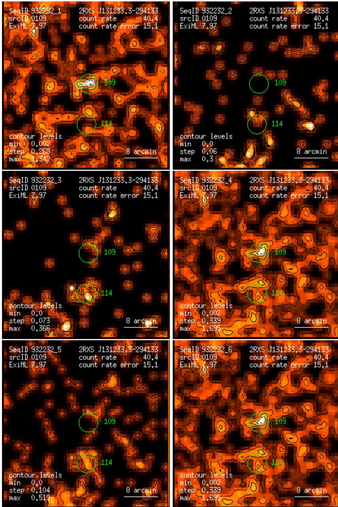
Figure 109: RASS 932232: detection 0109: band rate images, Gaussian filter: (1) PSPC channels 11 – 41, (2) 52 – 90, (3) 91 – 201, (4) 11 – 235, (5) 52 – 201, (6) 11 – 201. Broad band rates in counts/ks. Band rate contour levels in counts/ks/arcmin 2 .
