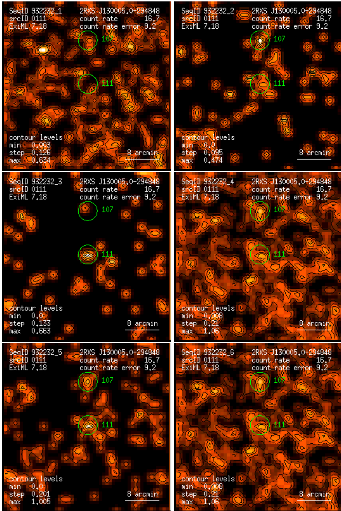
Figure 111: RASS 932232: detection 0111: band rate images, Gaussian filter: (1) PSPC channels 11 – 41, (2) 52 – 90, (3) 91 – 201, (4) 11 – 235, (5) 52 – 201, (6) 11 – 201. Broad band rates in counts/ks. Band rate contour levels in counts/ks/arcmin 2 .
