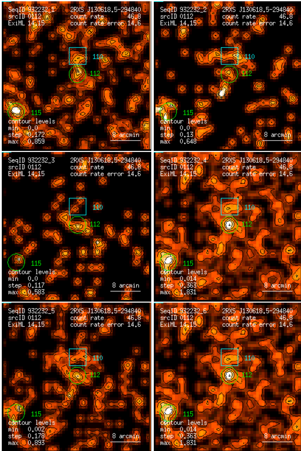
Figure 112: RASS 932232: detection 0112: band rate images, Gaussian filter: (1) PSPC channels 11 – 41, (2) 52 – 90, (3) 91 – 201, (4) 11 – 235, (5) 52 – 201, (6) 11 – 201. Broad band rates in counts/ks. Band rate contour levels in counts/ks/arcmin 2 .
