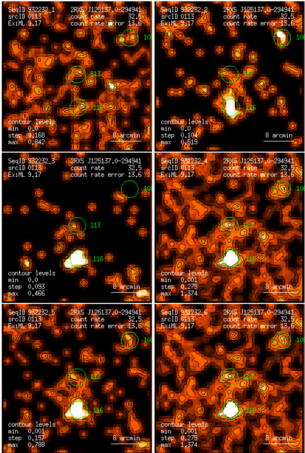
Figure 113: RASS 932232: detection 0113: band rate images, Gaussian filter: (1) PSPC channels 11 – 41, (2) 52 – 90, (3) 91 – 201, (4) 11 – 235, (5) 52 – 201, (6) 11 – 201. Broad band rates in counts/ks. Band rate contour levels in counts/ks/arcmin 2 .
