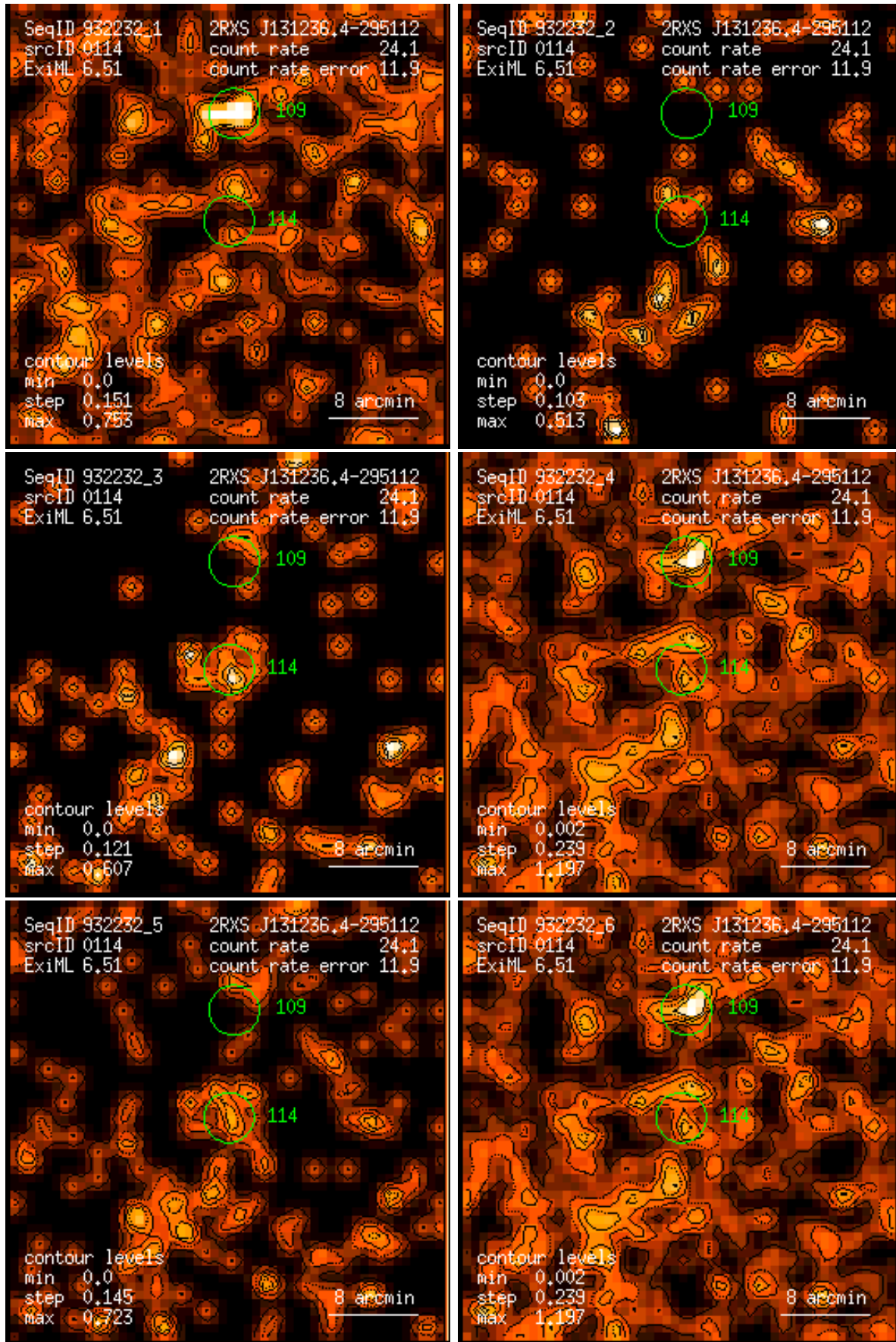
Figure 114: RASS 932232: detection 0114: band rate images, Gaussian filter: (1) PSPC channels 11 – 41, (2) 52 – 90, (3) 91 – 201, (4) 11 – 235, (5) 52 – 201, (6) 11 – 201. Broad band rates in counts/ks. Band rate contour levels in counts/ks/arcmin 2 .
