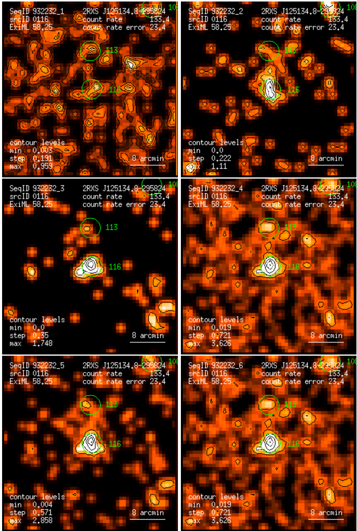
Figure 116: RASS 932232: detection 0116: band rate images, Gaussian filter: (1) PSPC channels 11 – 41, (2) 52 – 90, (3) 91 – 201, (4) 11 – 235, (5) 52 – 201, (6) 11 – 201. Broad band rates in counts/ks. Band rate contour levels in counts/ks/arcmin 2 .
