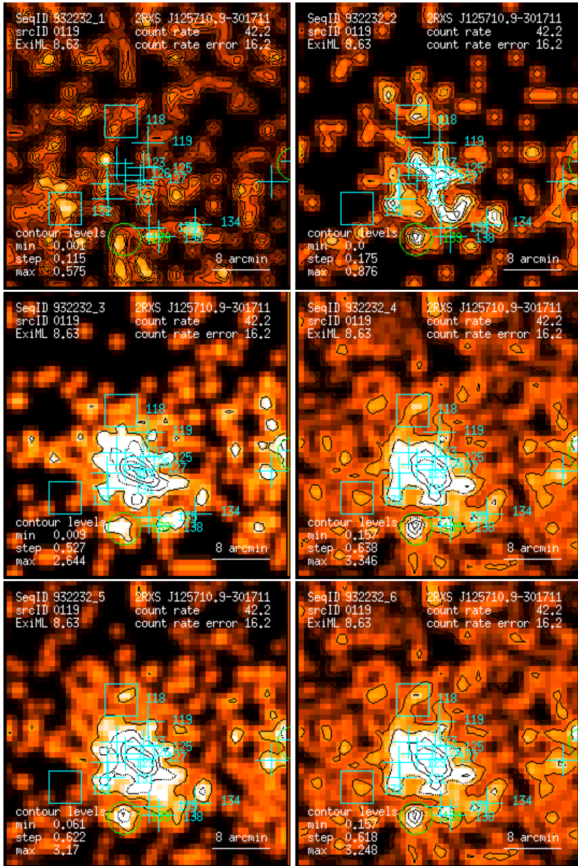
Figure 119: RASS 932232: detection 0119: band rate images, Gaussian filter: (1) PSPC channels 11 – 41, (2) 52 – 90, (3) 91 – 201, (4) 11 – 235, (5) 52 – 201, (6) 11 – 201. Broad band rates in counts/ks. Band rate contour levels in counts/ks/arcmin 2 .
