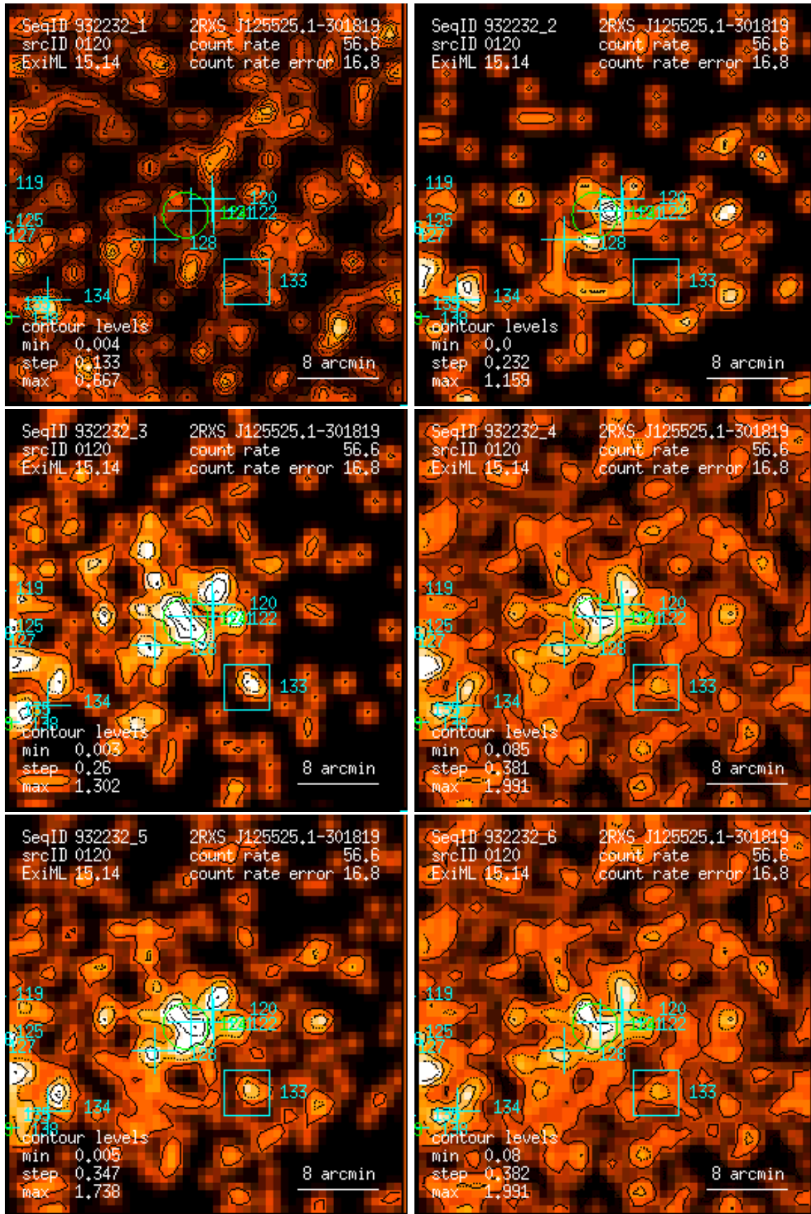
Figure 120: RASS 932232: detection 0120: band rate images, Gaussian filter: (1) PSPC channels 11 – 41, (2) 52 – 90, (3) 91 – 201, (4) 11 – 235, (5) 52 – 201, (6) 11 – 201. Broad band rates in counts/ks. Band rate contour levels in counts/ks/arcmin 2 .
