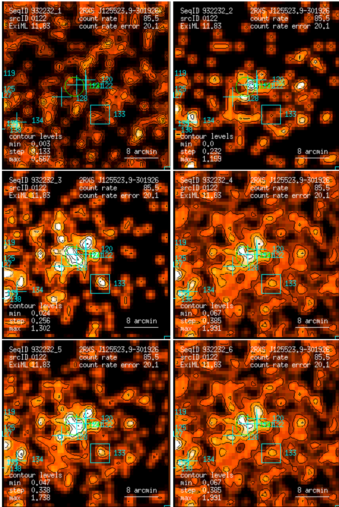
Figure 122: RASS 932232: detection 0122: band rate images, Gaussian filter: (1) PSPC channels 11 – 41, (2) 52 – 90, (3) 91 – 201, (4) 11 – 235, (5) 52 – 201, (6) 11 – 201. Broad band rates in counts/ks. Band rate contour levels in counts/ks/arcmin 2 .
