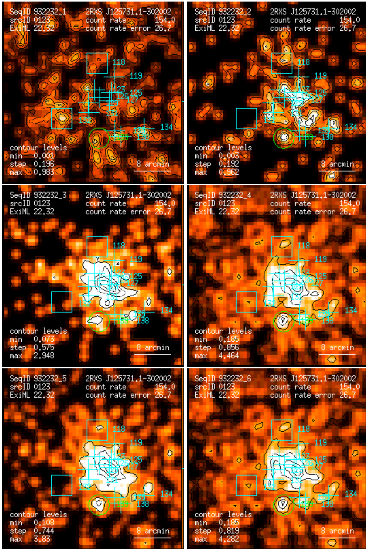
Figure 123: RASS 932232: detection 0123: band rate images, Gaussian filter: (1) PSPC channels 11 – 41, (2) 52 – 90, (3) 91 – 201, (4) 11 – 235, (5) 52 – 201, (6) 11 – 201. Broad band rates in counts/ks. Band rate contour levels in counts/ks/arcmin 2 .
