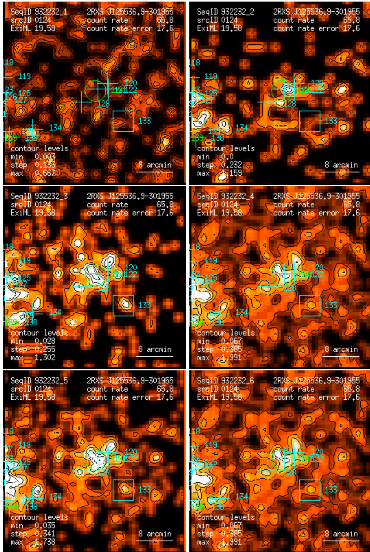
Figure 124: RASS 932232: detection 0124: band rate images, Gaussian filter: (1) PSPC channels 11 – 41, (2) 52 – 90, (3) 91 – 201, (4) 11 – 235, (5) 52 – 201, (6) 11 – 201. Broad band rates in counts/ks. Band rate contour levels in counts/ks/arcmin 2 .
