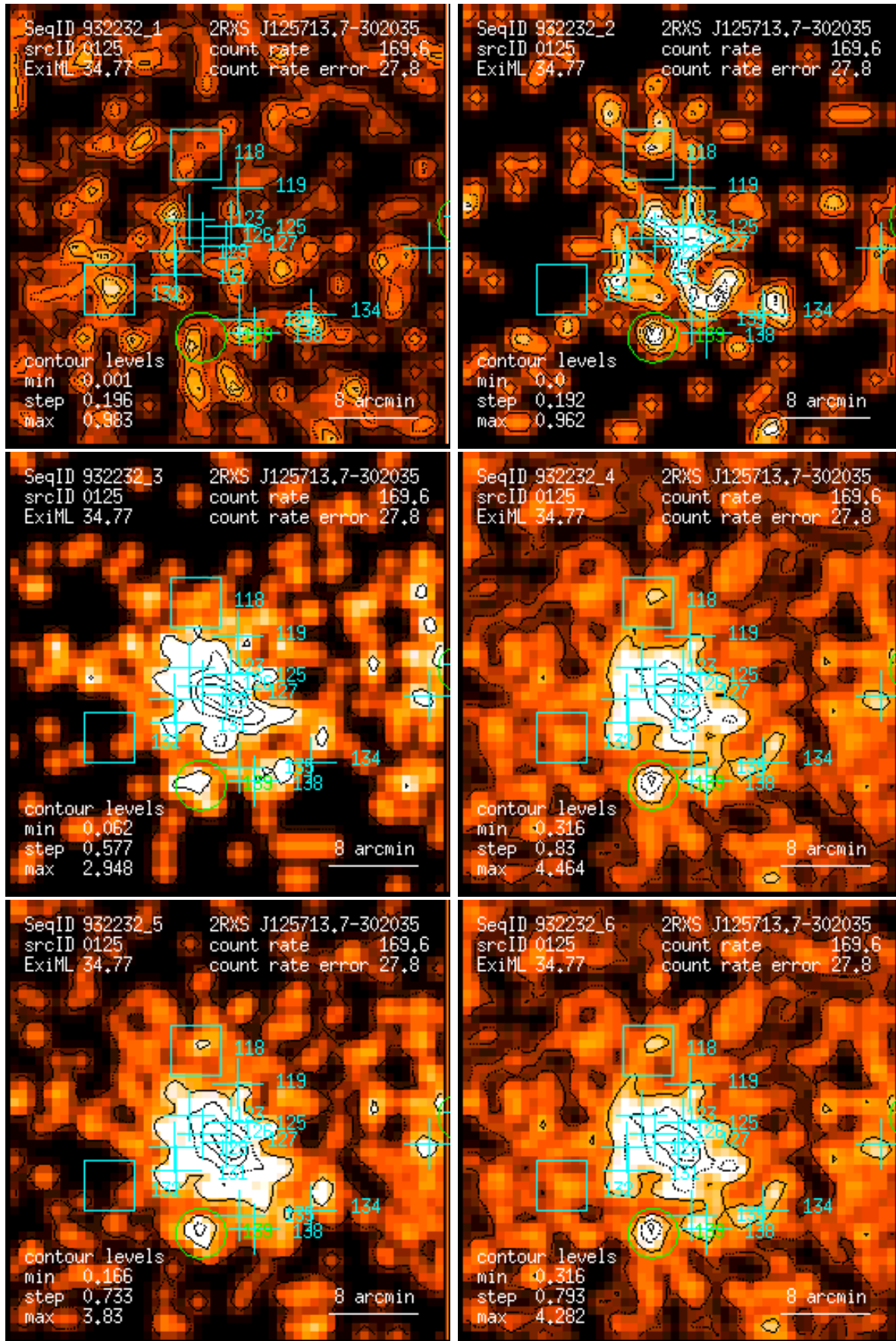
Figure 125: RASS 932232: detection 0125: band rate images, Gaussian filter: (1) PSPC channels 11 – 41, (2) 52 – 90, (3) 91 – 201, (4) 11 – 235, (5) 52 – 201, (6) 11 – 201. Broad band rates in counts/ks. Band rate contour levels in counts/ks/arcmin 2 .
