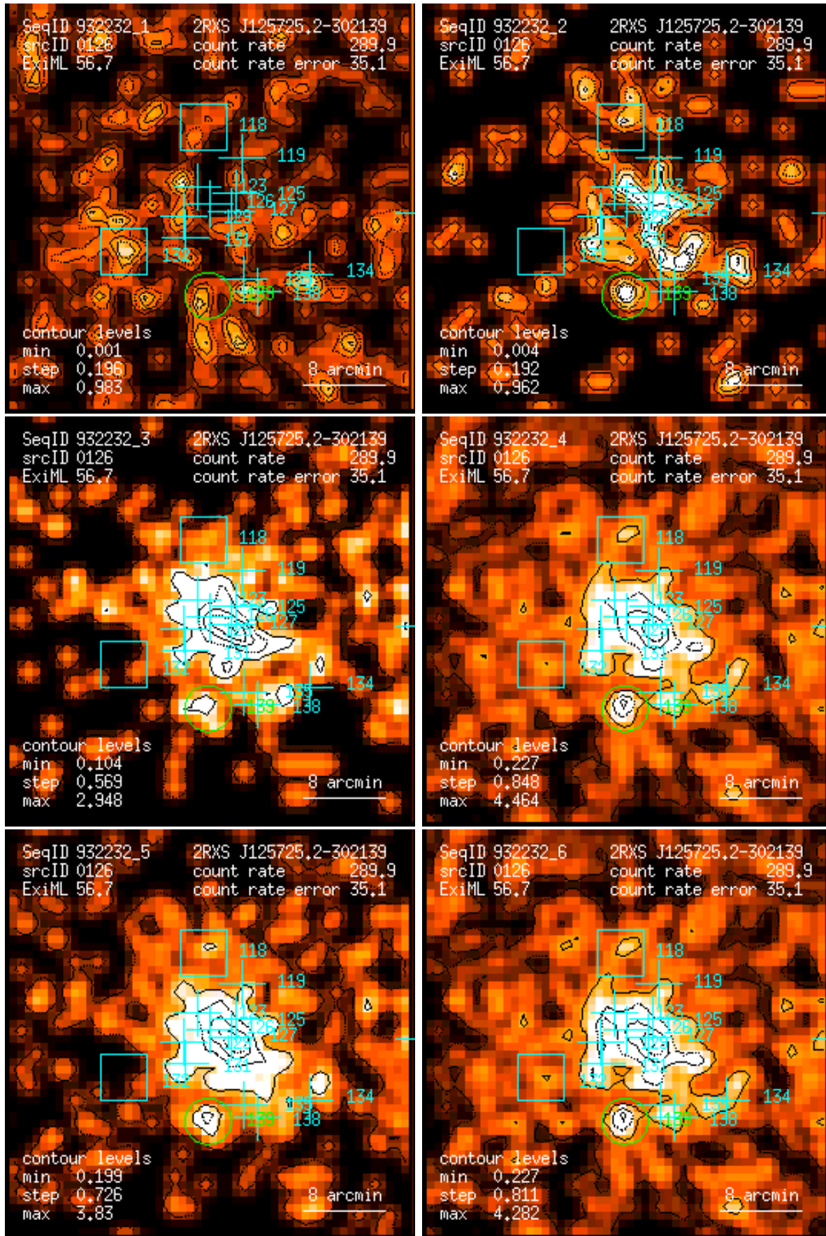
Figure 126: RASS 932232: detection 0126: band rate images, Gaussian filter: (1) PSPC channels 11 – 41, (2) 52 – 90, (3) 91 – 201, (4) 11 – 235, (5) 52 – 201, (6) 11 – 201. Broad band rates in counts/ks. Band rate contour levels in counts/ks/arcmin 2 .
