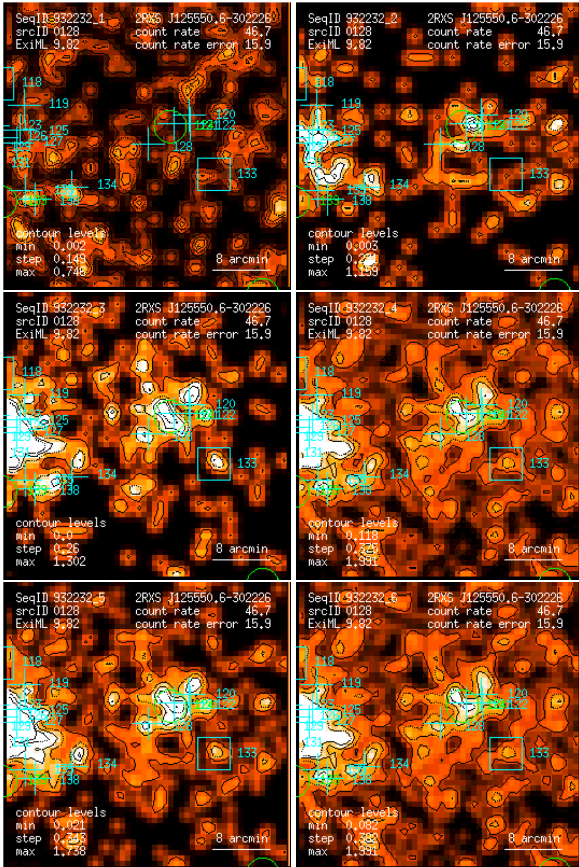
Figure 128: RASS 932232: detection 0128: band rate images, Gaussian filter: (1) PSPC channels 11 – 41, (2) 52 – 90, (3) 91 – 201, (4) 11 – 235, (5) 52 – 201, (6) 11 – 201. Broad band rates in counts/ks. Band rate contour levels in counts/ks/arcmin 2 .
