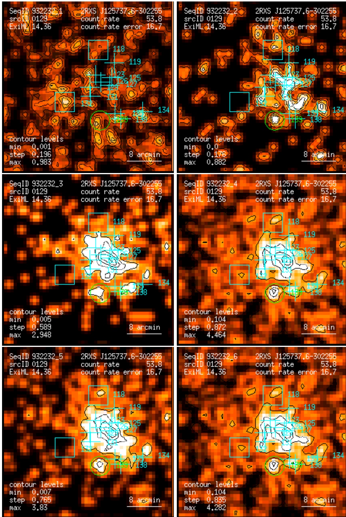
Figure 129: RASS 932232: detection 0129: band rate images, Gaussian filter: (1) PSPC channels 11 – 41, (2) 52 – 90, (3) 91 – 201, (4) 11 – 235, (5) 52 – 201, (6) 11 – 201. Broad band rates in counts/ks. Band rate contour levels in counts/ks/arcmin 2 .
