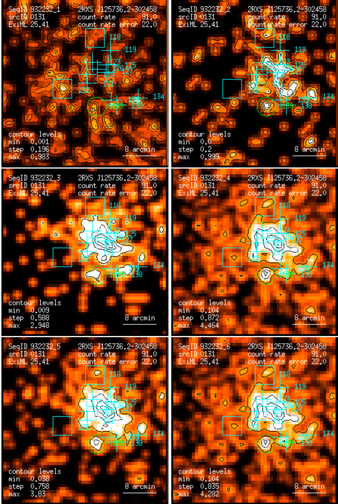
Figure 131: RASS 932232: detection 0131: band rate images, Gaussian filter: (1) PSPC channels 11 – 41, (2) 52 – 90, (3) 91 – 201, (4) 11 – 235, (5) 52 – 201, (6) 11 – 201. Broad band rates in counts/ks. Band rate contour levels in counts/ks/arcmin 2 .
