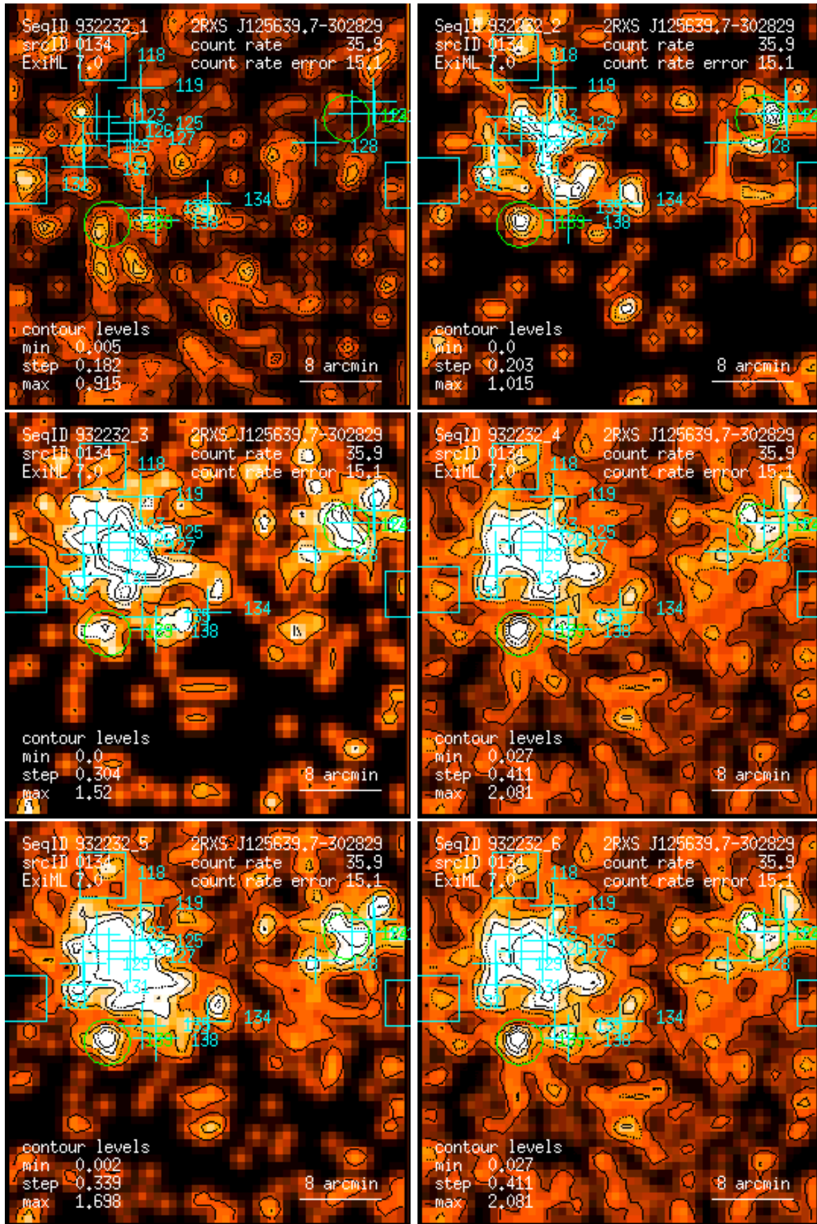
Figure 134: RASS 932232: detection 0134: band rate images, Gaussian filter: (1) PSPC channels 11 – 41, (2) 52 – 90, (3) 91 – 201, (4) 11 – 235, (5) 52 – 201, (6) 11 – 201. Broad band rates in counts/ks. Band rate contour levels in counts/ks/arcmin 2 .
