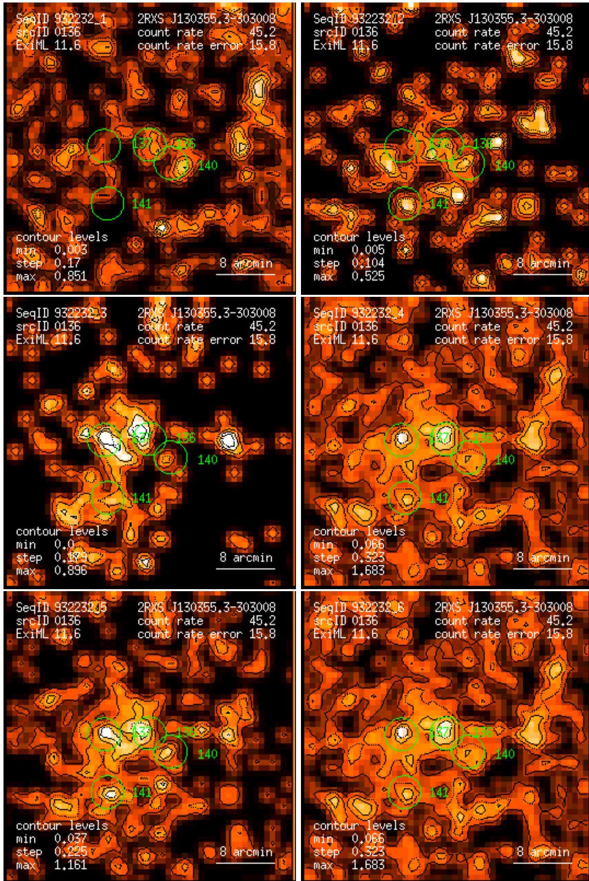
Figure 136: RASS 932232: detection 0136: band rate images, Gaussian filter: (1) PSPC channels 11 – 41, (2) 52 – 90, (3) 91 – 201, (4) 11 – 235, (5) 52 – 201, (6) 11 – 201. Broad band rates in counts/ks. Band rate contour levels in counts/ks/arcmin 2 .
