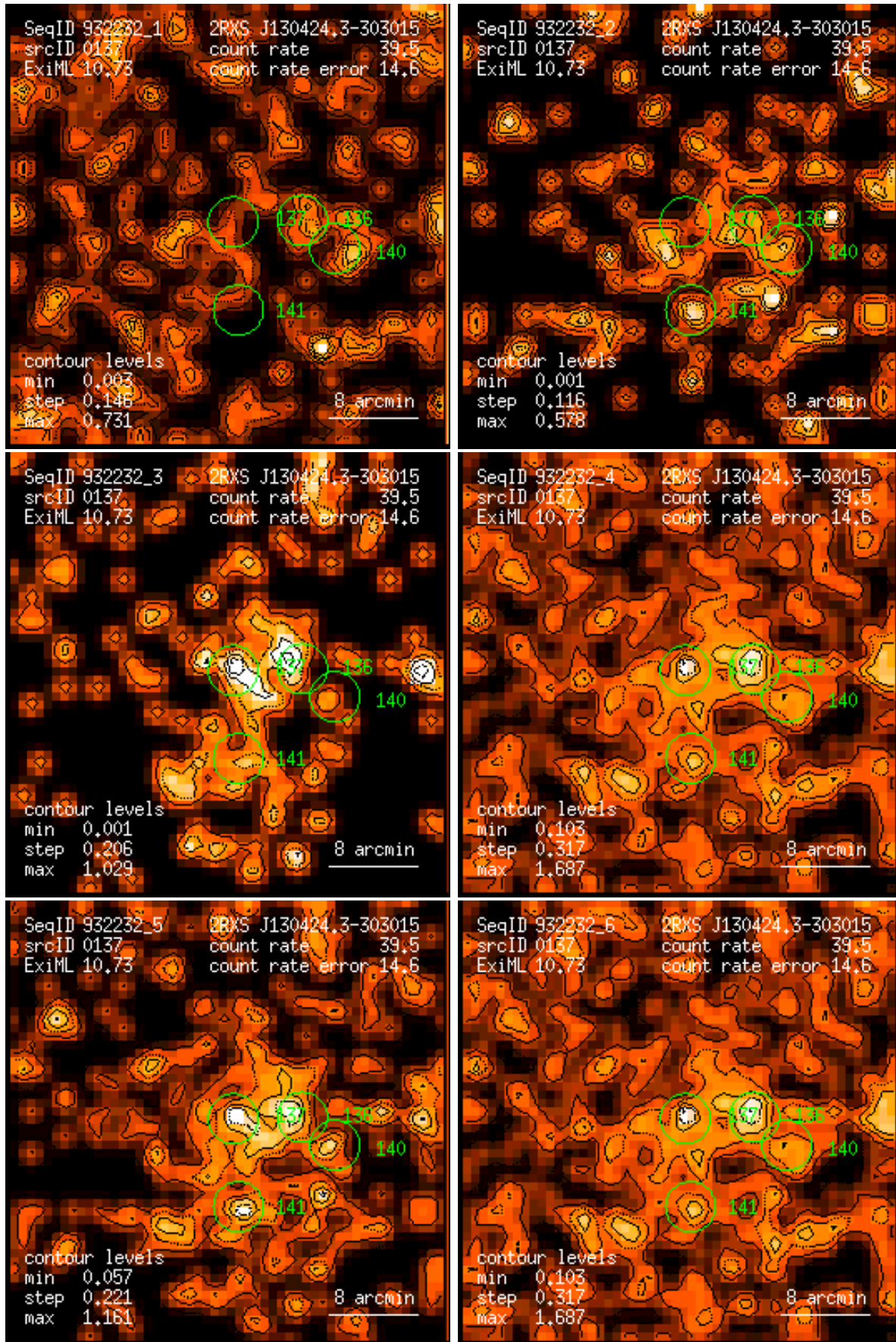
Figure 137: RASS 932232: detection 0137: band rate images, Gaussian filter: (1) PSPC channels 11 – 41, (2) 52 – 90, (3) 91 – 201, (4) 11 – 235, (5) 52 – 201, (6) 11 – 201. Broad band rates in counts/ks. Band rate contour levels in counts/ks/arcmin 2 .
