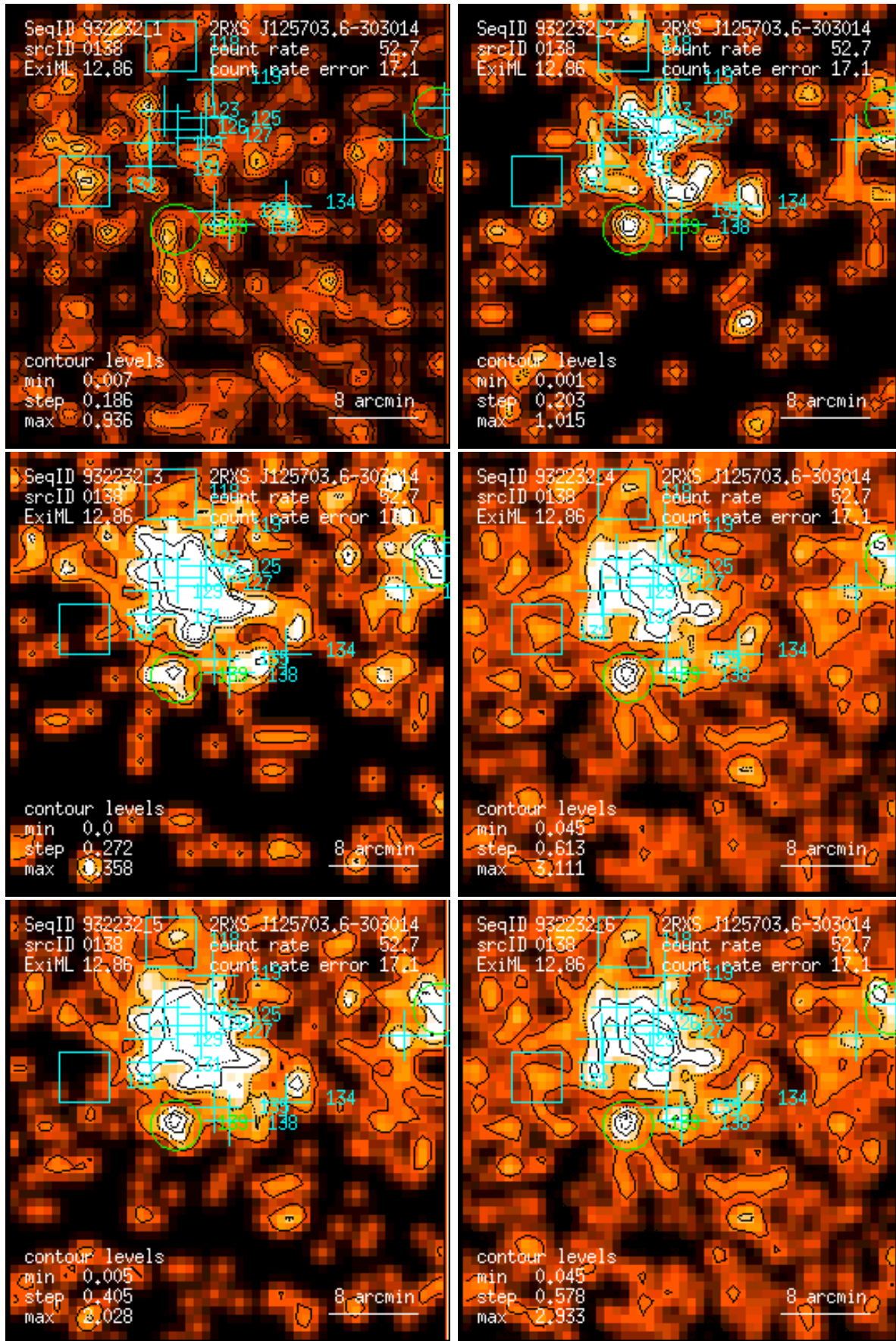
Figure 138: RASS 932232: detection 0138: band rate images, Gaussian filter: (1) PSPC channels 11 – 41, (2) 52 – 90, (3) 91 – 201, (4) 11 – 235, (5) 52 – 201, (6) 11 – 201. Broad band rates in counts/ks. Band rate contour levels in counts/ks/arcmin 2 .
