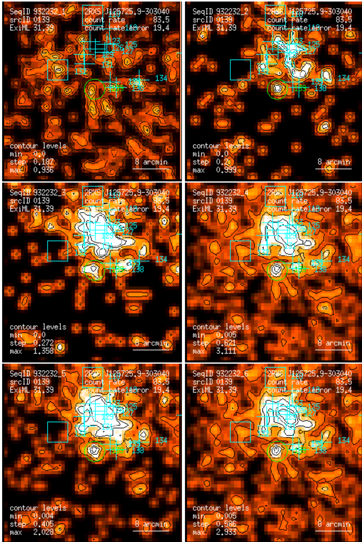
Figure 139: RASS 932232: detection 0139: band rate images, Gaussian filter: (1) PSPC channels 11 – 41, (2) 52 – 90, (3) 91 – 201, (4) 11 – 235, (5) 52 – 201, (6) 11 – 201. Broad band rates in counts/ks. Band rate contour levels in counts/ks/arcmin 2 .
