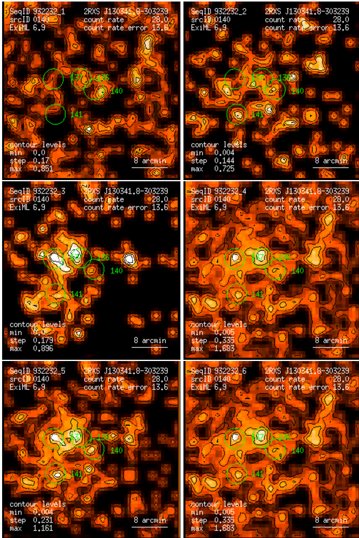
Figure 140: RASS 932232: detection 0140: band rate images, Gaussian filter: (1) PSPC channels 11 – 41, (2) 52 – 90, (3) 91 – 201, (4) 11 – 235, (5) 52 – 201, (6) 11 – 201. Broad band rates in counts/ks. Band rate contour levels in counts/ks/arcmin 2 .
