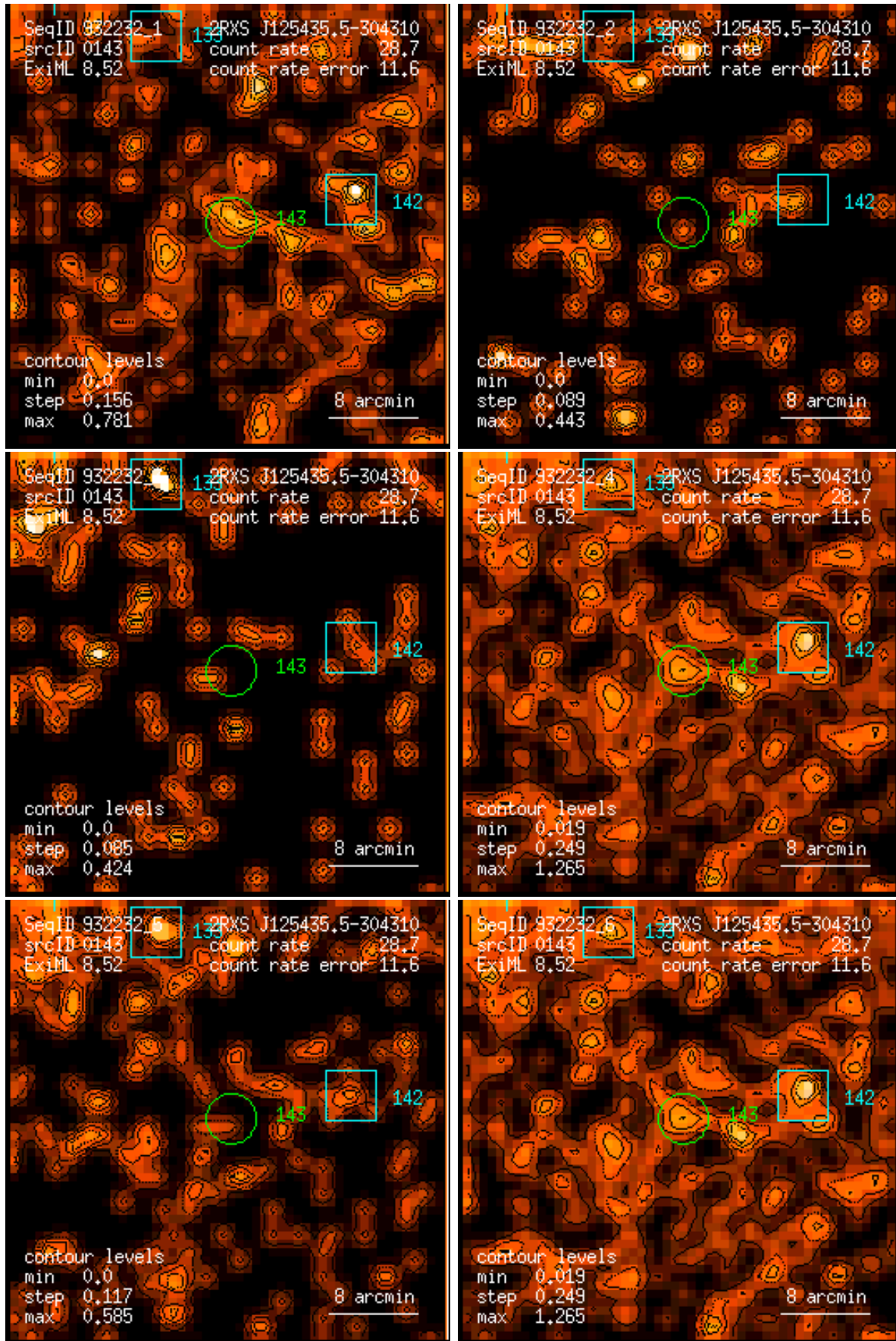
Figure 143: RASS 932232: detection 0143: band rate images, Gaussian filter: (1) PSPC channels 11 – 41, (2) 52 – 90, (3) 91 – 201, (4) 11 – 235, (5) 52 – 201, (6) 11 – 201. Broad band rates in counts/ks. Band rate contour levels in counts/ks/arcmin 2 .
