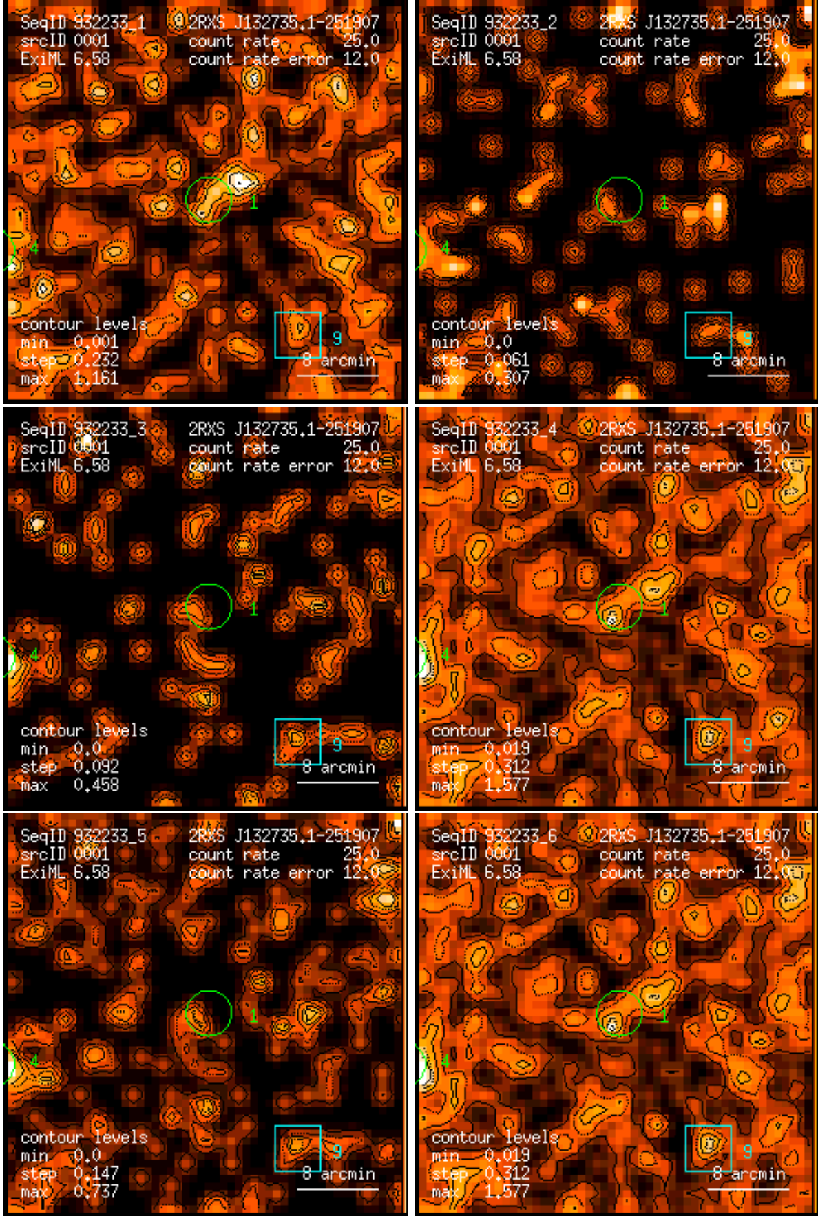
Figure 1: RASS 932233: detection 0001: band rate images, Gaussian filter: (1) PSPC channels 11 – 41, (2) 52 – 90, (3) 91 – 201, (4) 11 – 235, (5) 52 – 201, (6) 11 – 201. Broad band rates in counts/ks. Band rate contour levels in counts/ks/arcmin 2 .
