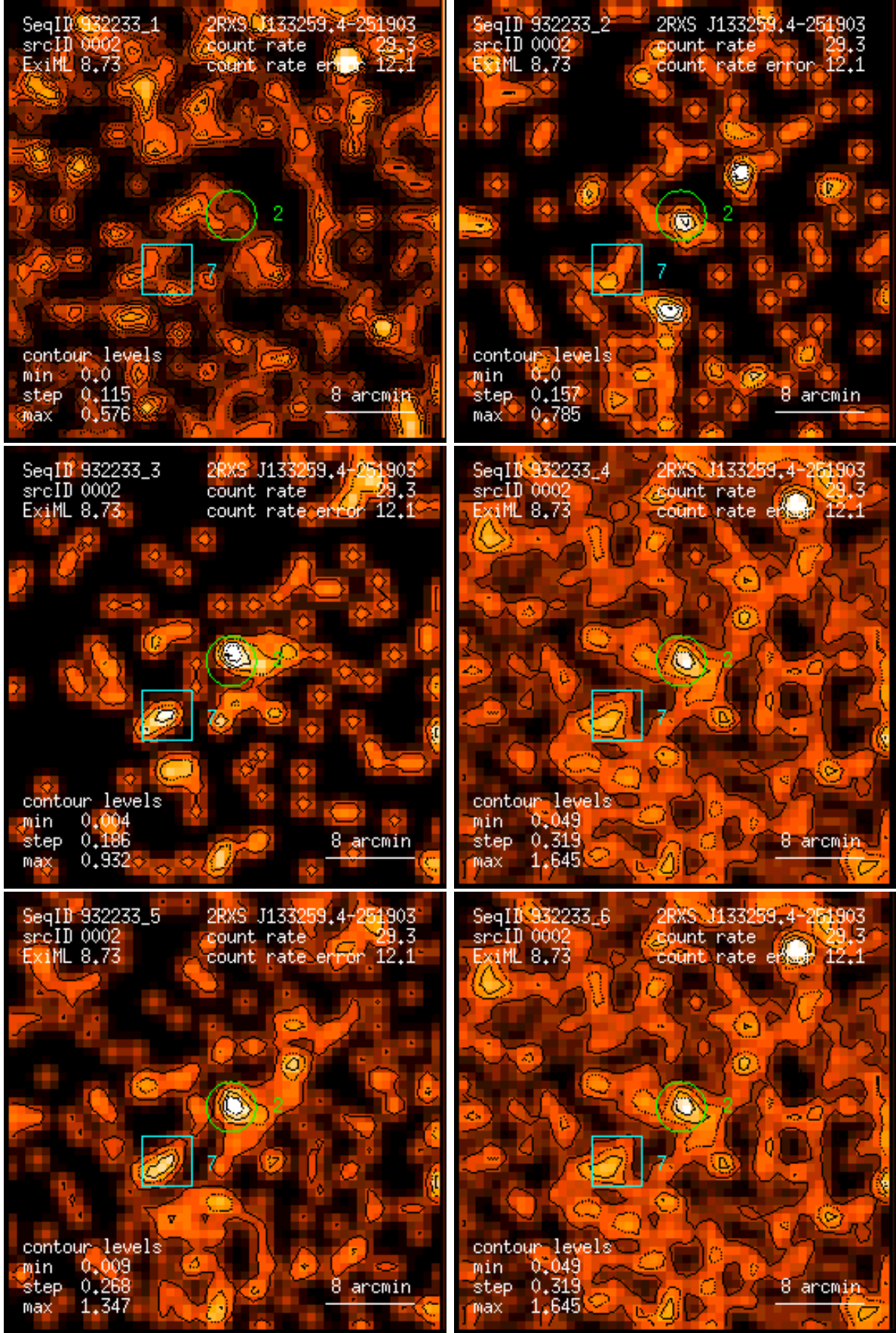
Figure 2: RASS 932233: detection 0002: band rate images, Gaussian filter: (1) PSPC channels 11 – 41, (2) 52 – 90, (3) 91 – 201, (4) 11 – 235, (5) 52 – 201, (6) 11 – 201. Broad band rates in counts/ks. Band rate contour levels in counts/ks/arcmin 2 .
