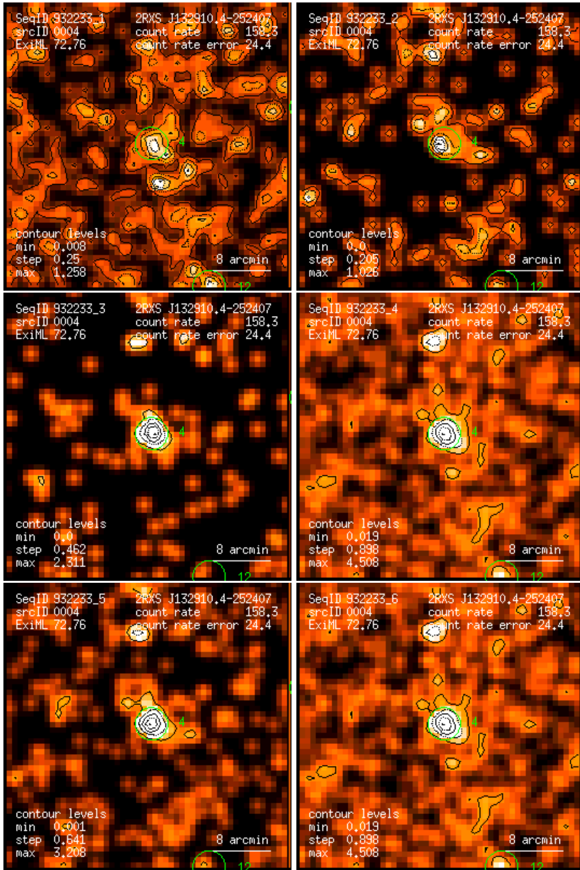
Figure 4: RASS 932233: detection 0004: band rate images, Gaussian filter: (1) PSPC channels 11 – 41, (2) 52 – 90, (3) 91 – 201, (4) 11 – 235, (5) 52 – 201, (6) 11 – 201. Broad band rates in counts/ks. Band rate contour levels in counts/ks/arcmin 2 .
