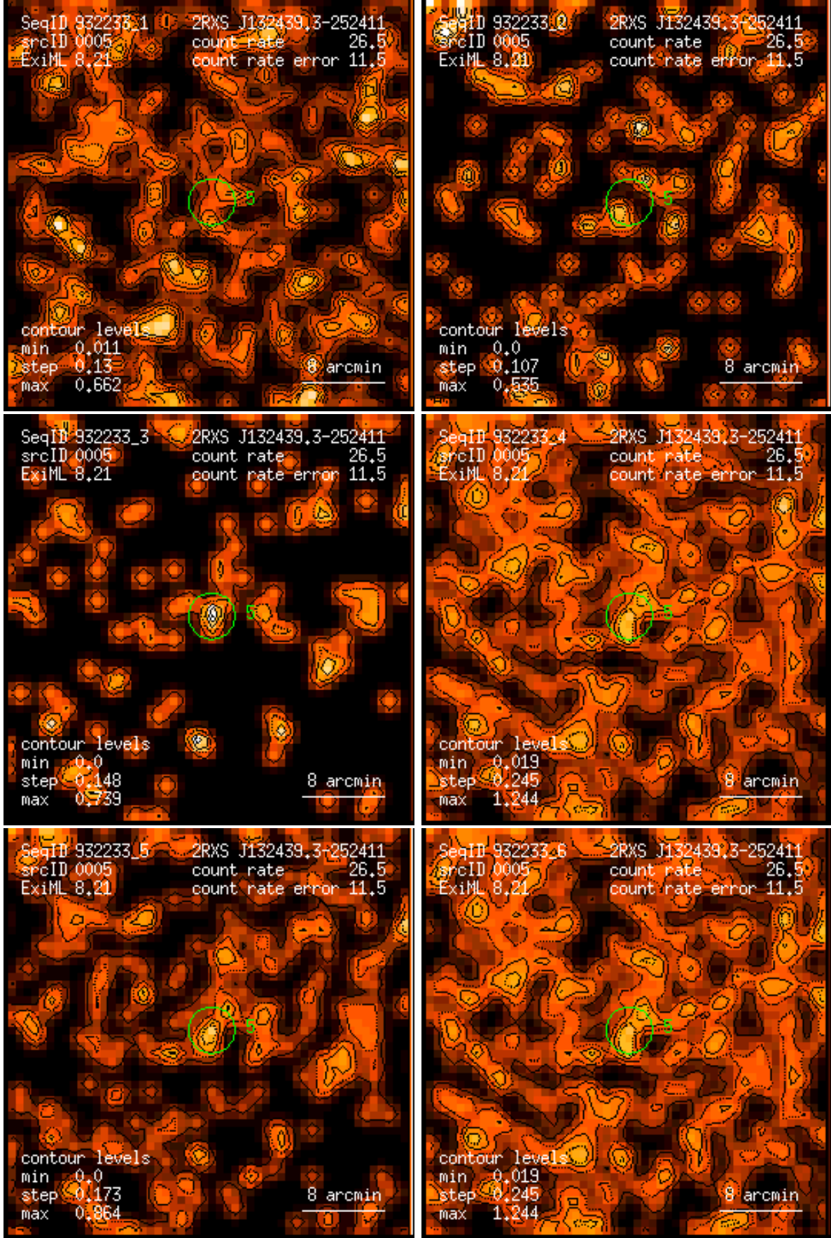
Figure 5: RASS 932233: detection 0005: band rate images, Gaussian filter: (1) PSPC channels 11 – 41, (2) 52 – 90, (3) 91 – 201, (4) 11 – 235, (5) 52 – 201, (6) 11 – 201. Broad band rates in counts/ks. Band rate contour levels in counts/ks/arcmin 2 .
