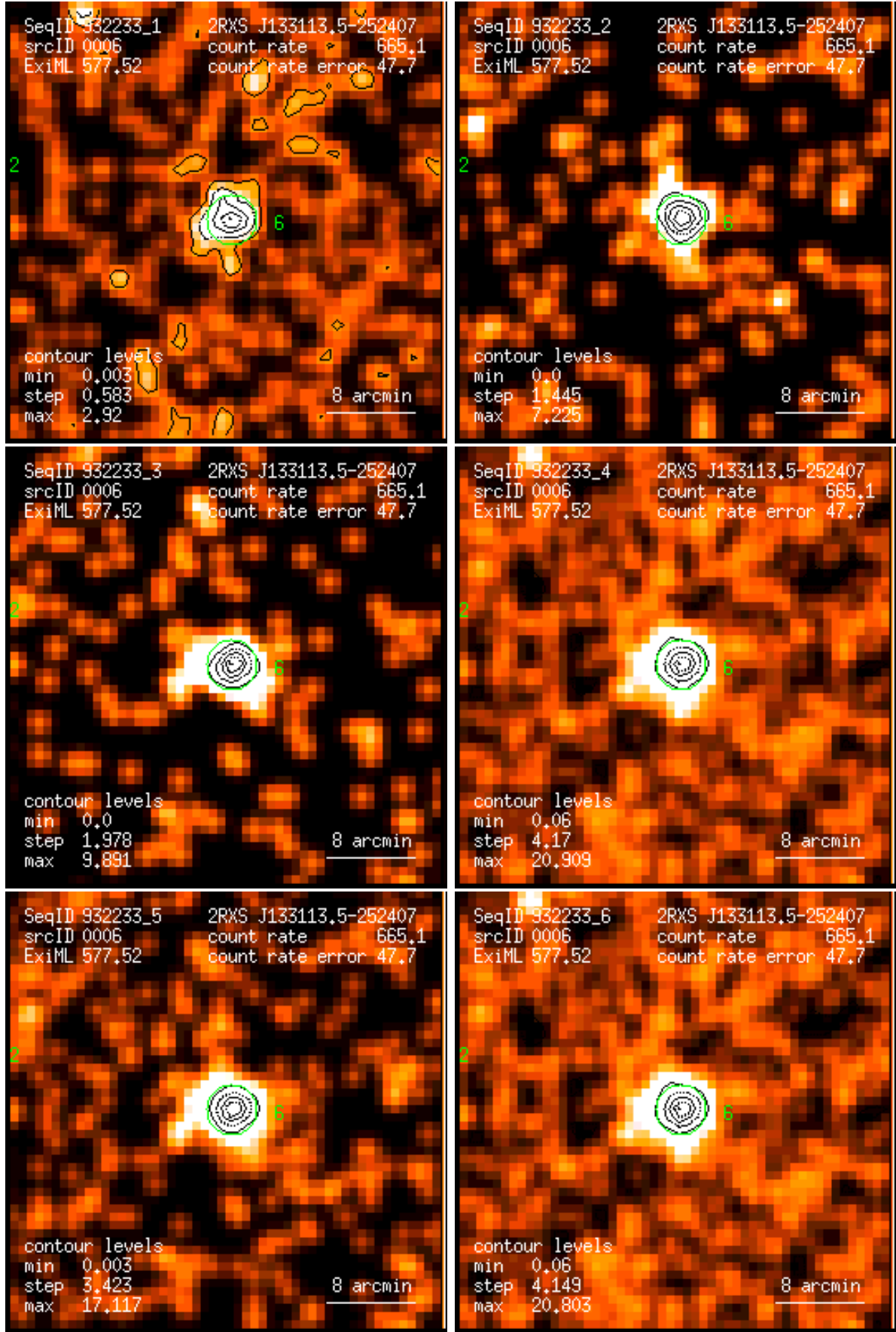
Figure 6: RASS 932233: detection 0006: band rate images, Gaussian filter: (1) PSPC channels 11 – 41, (2) 52 – 90, (3) 91 – 201, (4) 11 – 235, (5) 52 – 201, (6) 11 – 201. Broad band rates in counts/ks. Band rate contour levels in counts/ks/arcmin 2 .
