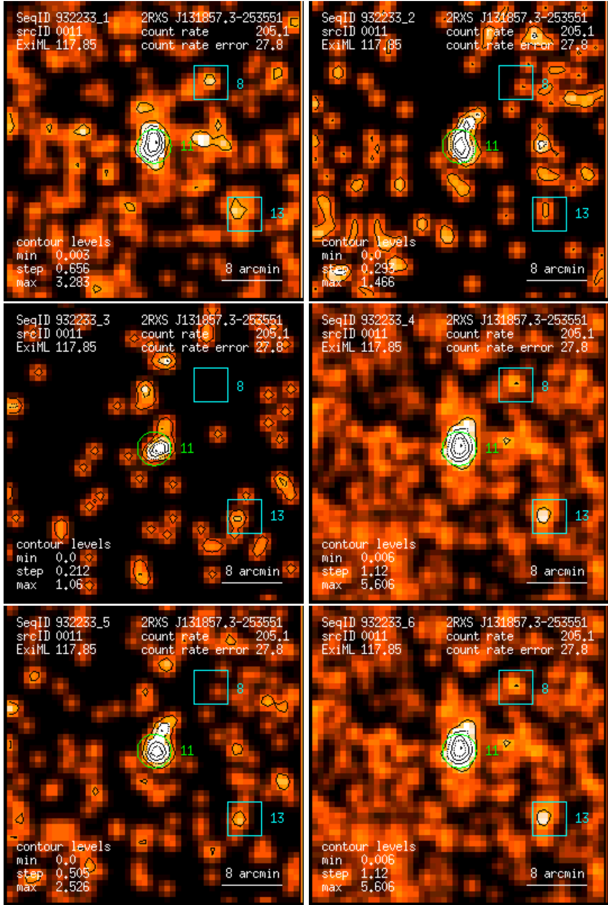
Figure 11: RASS 932233: detection 0011: band rate images, Gaussian filter: (1) PSPC channels 11 – 41, (2) 52 – 90, (3) 91 – 201, (4) 11 – 235, (5) 52 – 201, (6) 11 – 201. Broad band rates in counts/ks. Band rate contour levels in counts/ks/arcmin 2 .
