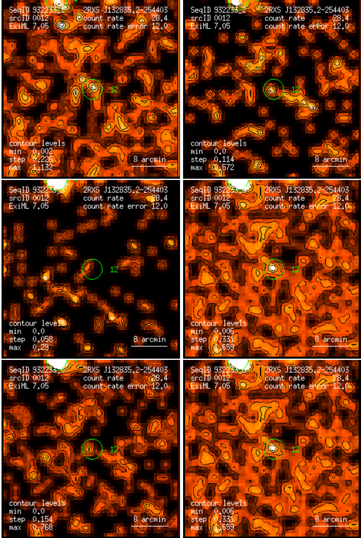
Figure 12: RASS 932233: detection 0012: band rate images, Gaussian filter: (1) PSPC channels 11 – 41, (2) 52 – 90, (3) 91 – 201, (4) 11 – 235, (5) 52 – 201, (6) 11 – 201. Broad band rates in counts/ks. Band rate contour levels in counts/ks/arcmin 2 .
