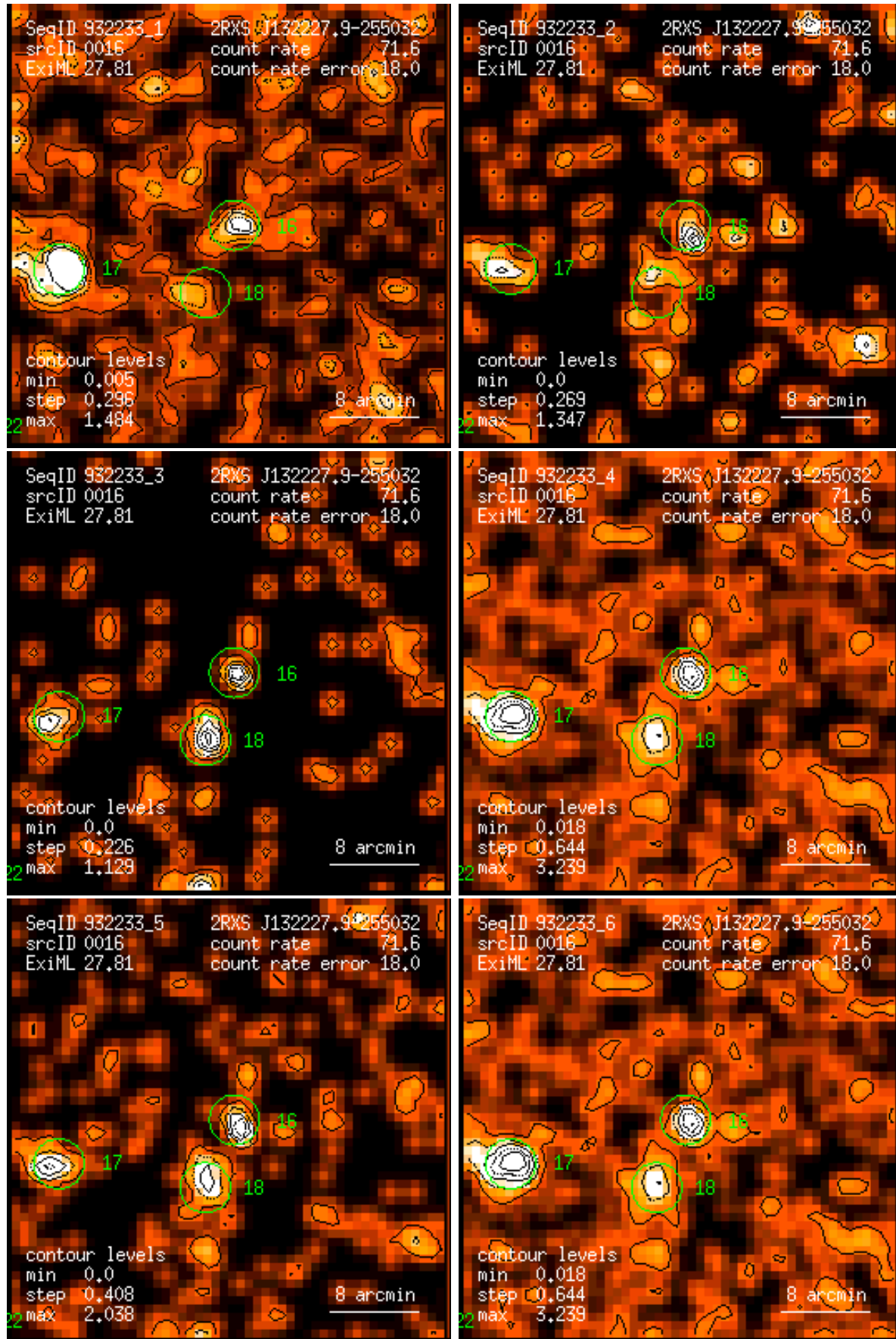
Figure 16: RASS 932233: detection 0016: band rate images, Gaussian filter: (1) PSPC channels 11 – 41, (2) 52 – 90, (3) 91 – 201, (4) 11 – 235, (5) 52 – 201, (6) 11 – 201. Broad band rates in counts/ks. Band rate contour levels in counts/ks/arcmin 2 .
