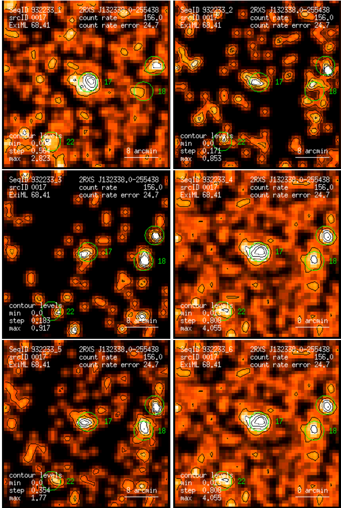
Figure 17: RASS 932233: detection 0017: band rate images, Gaussian filter: (1) PSPC channels 11 – 41, (2) 52 – 90, (3) 91 – 201, (4) 11 – 235, (5) 52 – 201, (6) 11 – 201. Broad band rates in counts/ks. Band rate contour levels in counts/ks/arcmin 2 .
