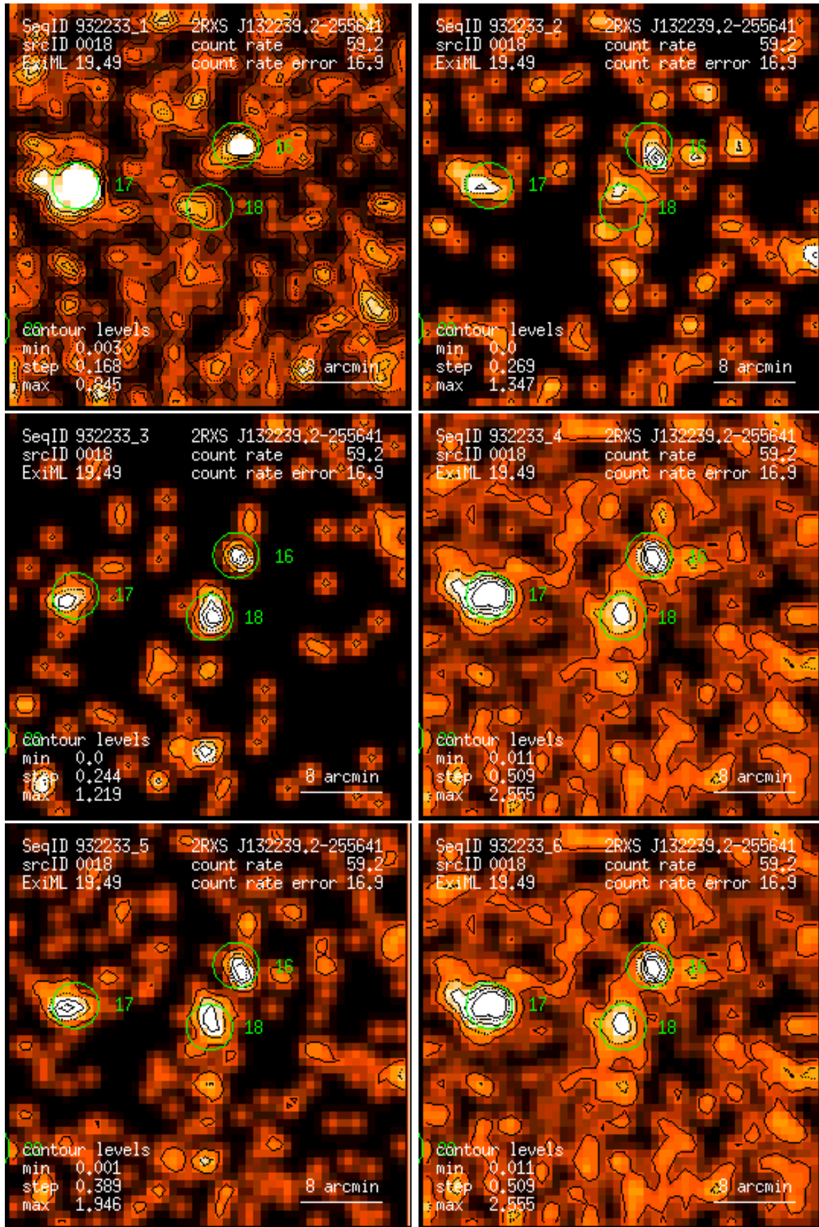
Figure 18: RASS 932233: detection 0018: band rate images, Gaussian filter: (1) PSPC channels 11 – 41, (2) 52 – 90, (3) 91 – 201, (4) 11 – 235, (5) 52 – 201, (6) 11 – 201. Broad band rates in counts/ks. Band rate contour levels in counts/ks/arcmin 2 .
