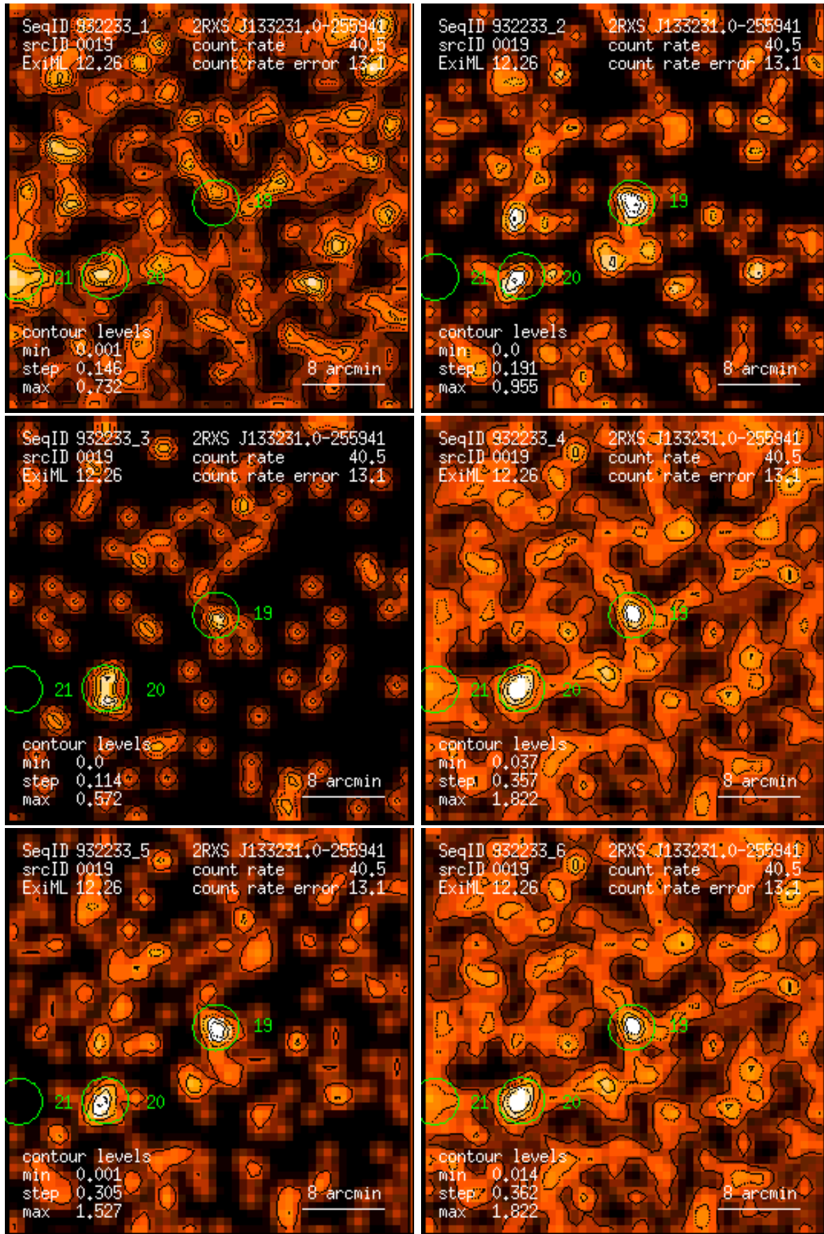
Figure 19: RASS 932233: detection 0019: band rate images, Gaussian filter: (1) PSPC channels 11 – 41, (2) 52 – 90, (3) 91 – 201, (4) 11 – 235, (5) 52 – 201, (6) 11 – 201. Broad band rates in counts/ks. Band rate contour levels in counts/ks/arcmin 2 .
