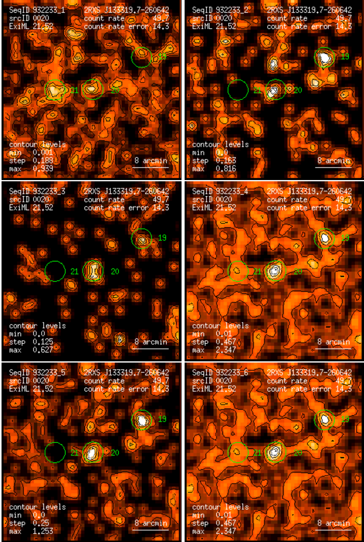
Figure 20: RASS 932233: detection 0020: band rate images, Gaussian filter: (1) PSPC channels 11 – 41, (2) 52 – 90, (3) 91 – 201, (4) 11 – 235, (5) 52 – 201, (6) 11 – 201. Broad band rates in counts/ks. Band rate contour levels in counts/ks/arcmin 2 .
