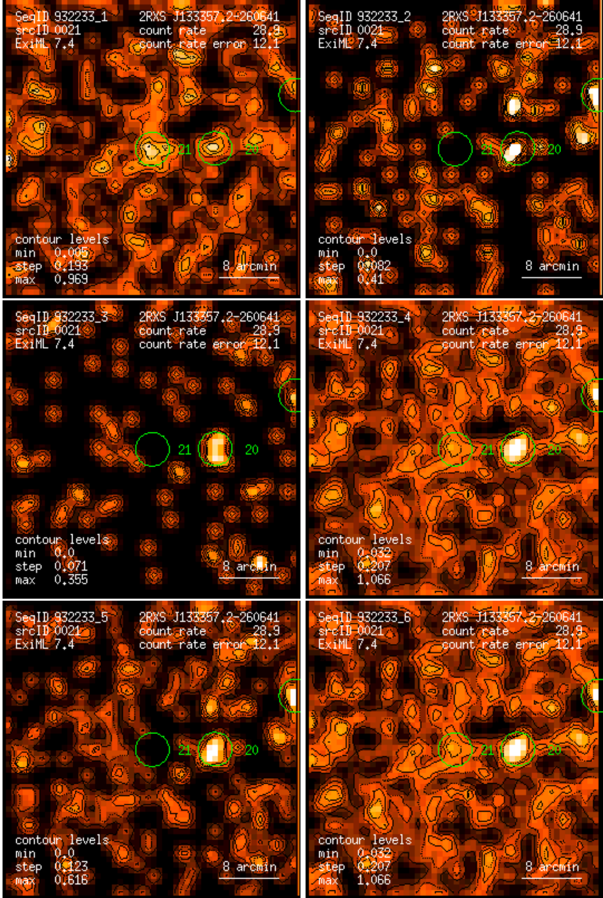
Figure 21: RASS 932233: detection 0021: band rate images, Gaussian filter: (1) PSPC channels 11 – 41, (2) 52 – 90, (3) 91 – 201, (4) 11 – 235, (5) 52 – 201, (6) 11 – 201. Broad band rates in counts/ks. Band rate contour levels in counts/ks/arcmin 2 .
